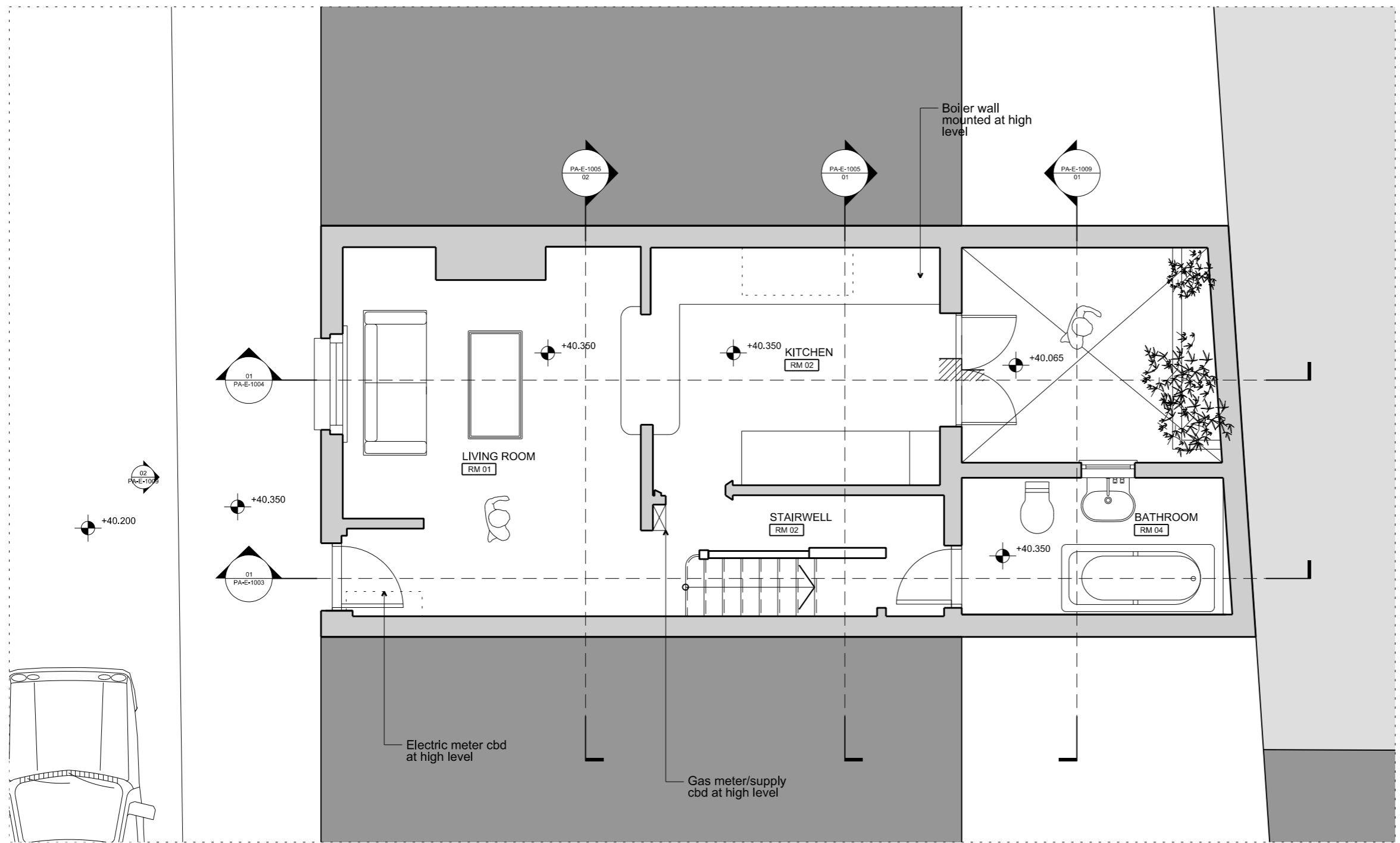
01 GROUND FLOOR PLAN 1:50
