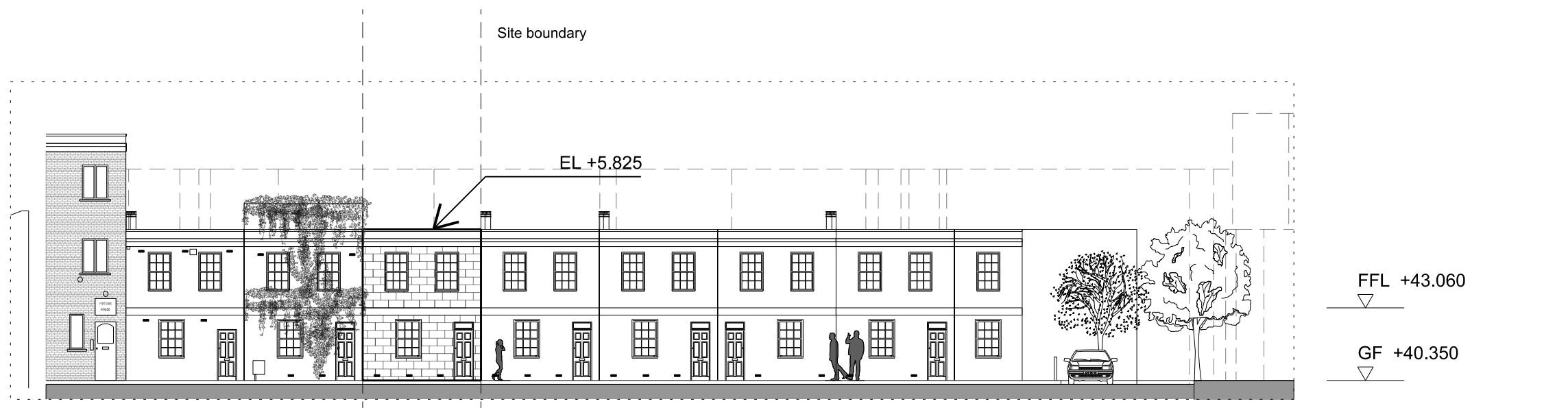
01 FRONT ELEVATION 1:200
