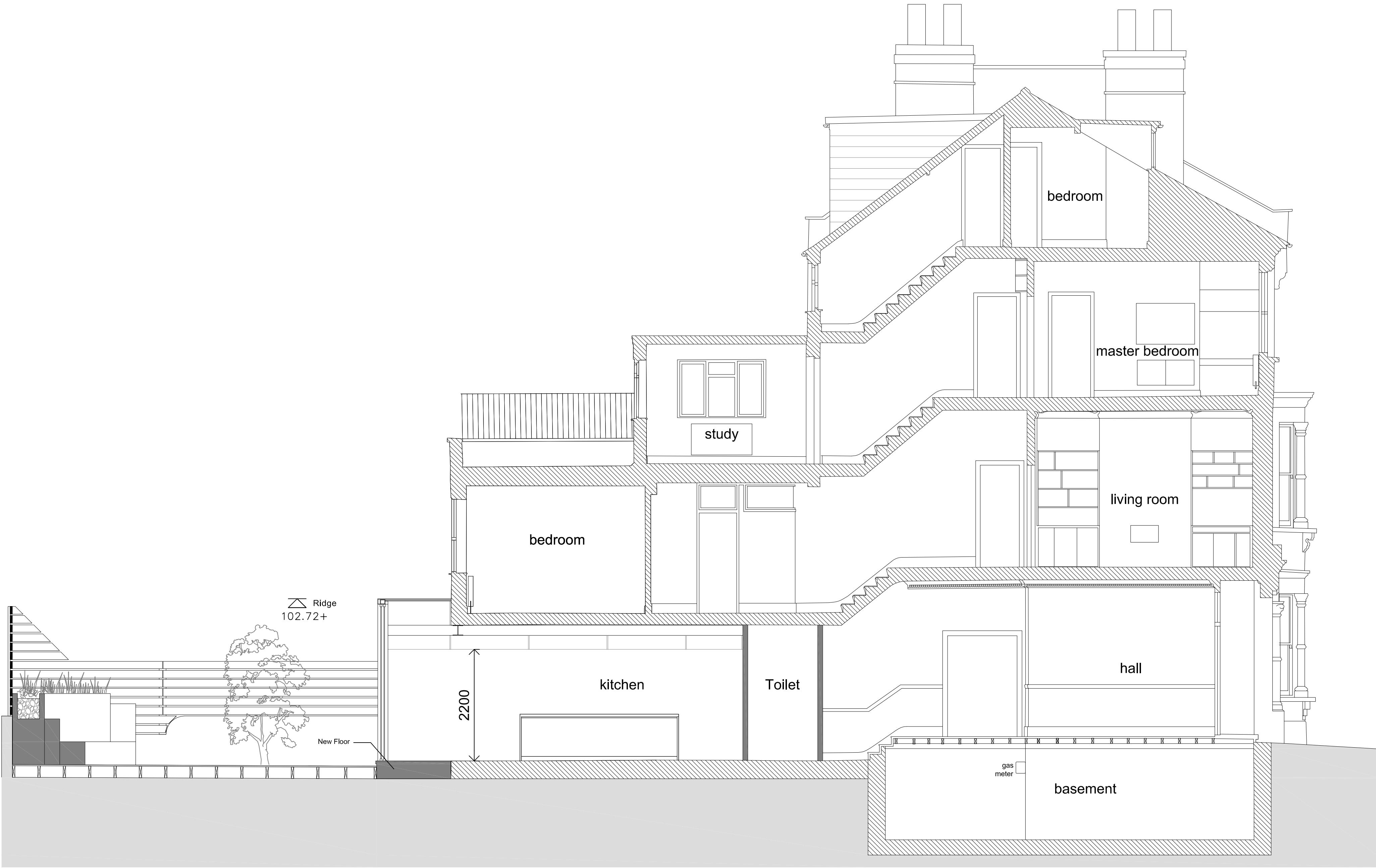
SECTION AA
