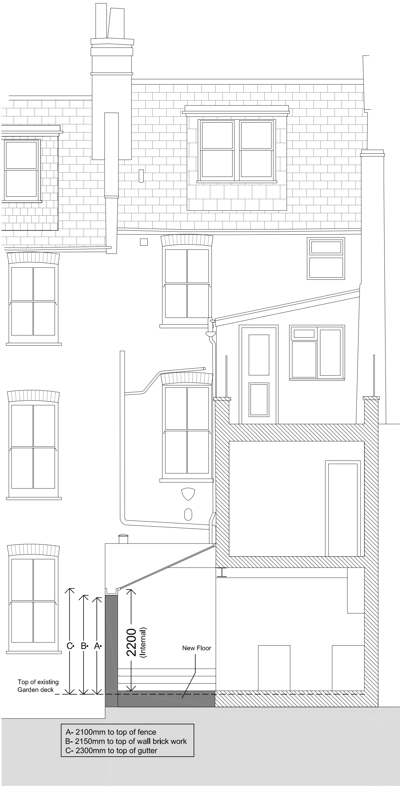
SECTION BB
