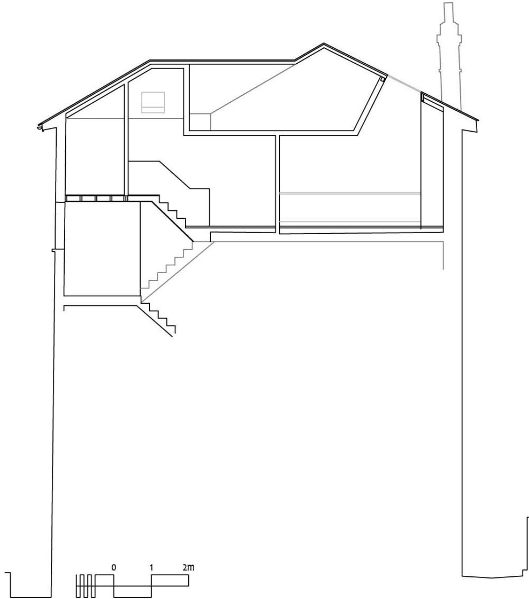
Section 2 – proposed
