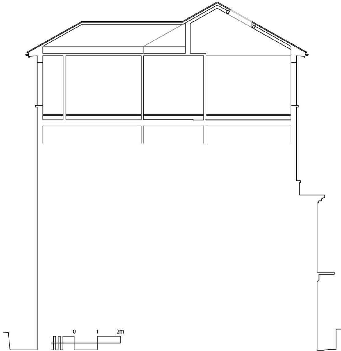
Section 1 – proposed
