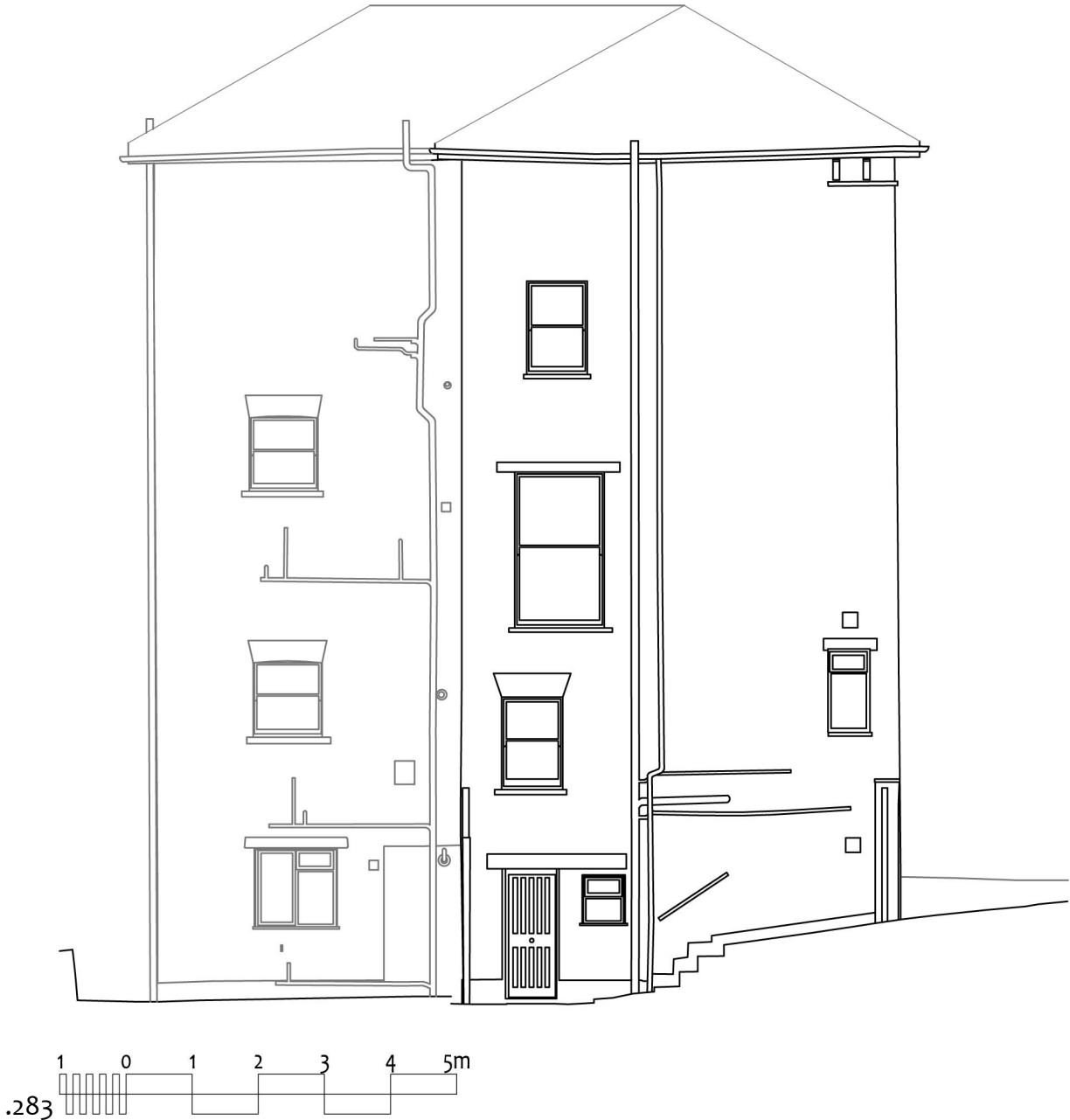
Side (North) Elevation – Existing
