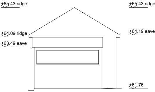
South elevation
