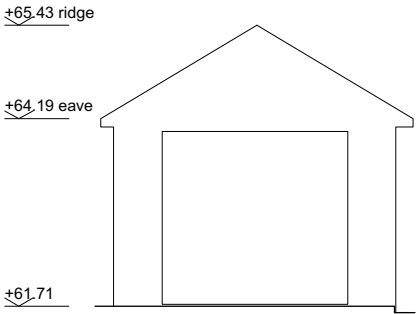
North elevation
