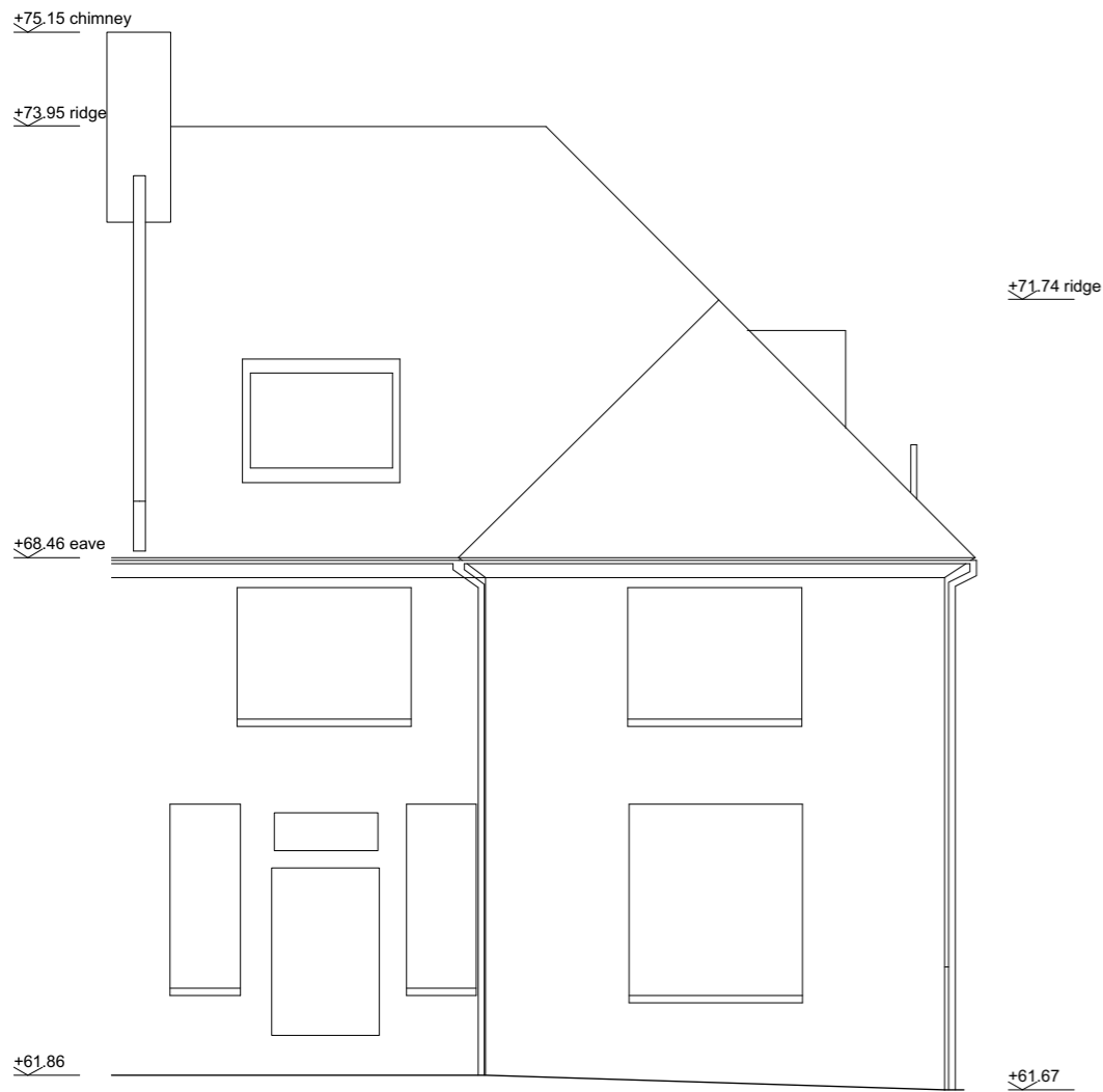
North elevation
