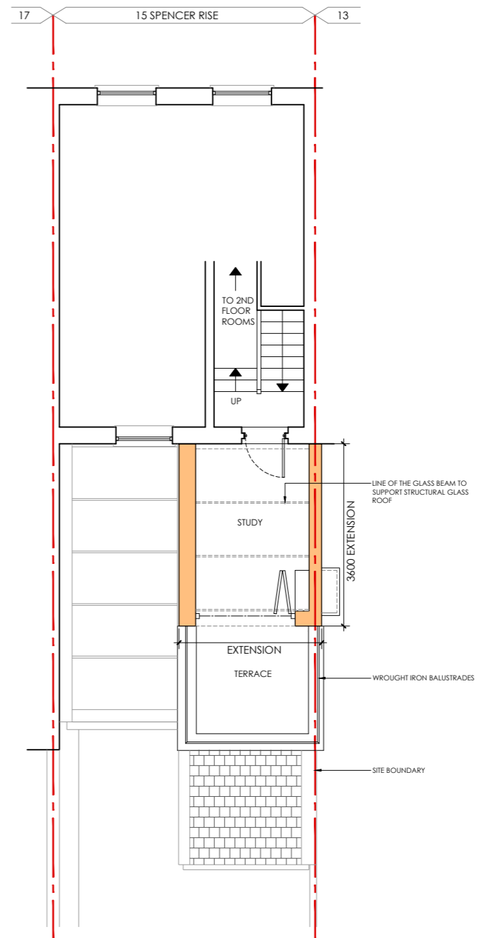
5 PLAN-MEZ/2nd FLOOR PROPOSED 1:100
