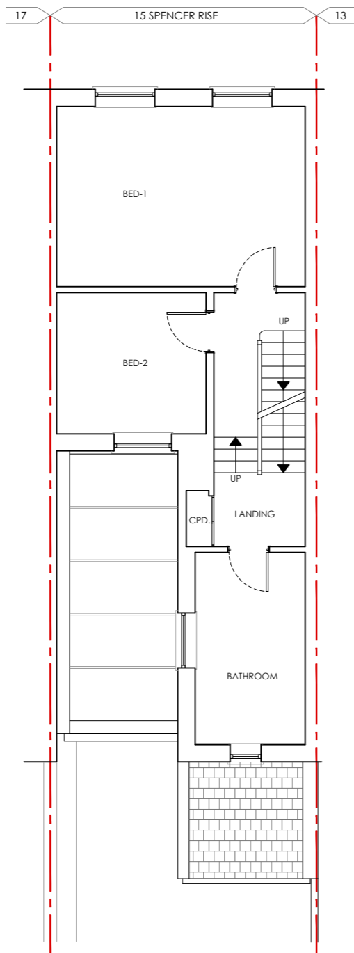
3 PLAN-FIRST FLOOR EXISTING 1:100
