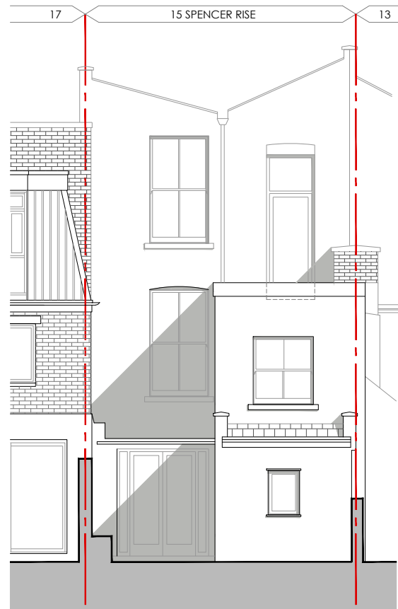
1 ELEVATION - REAR EXISTING 1:100
