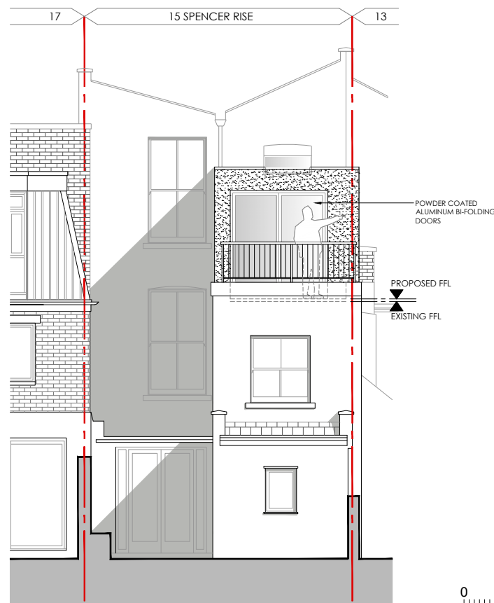
3 ELEVATION - REAR PROPOSED 1:100
