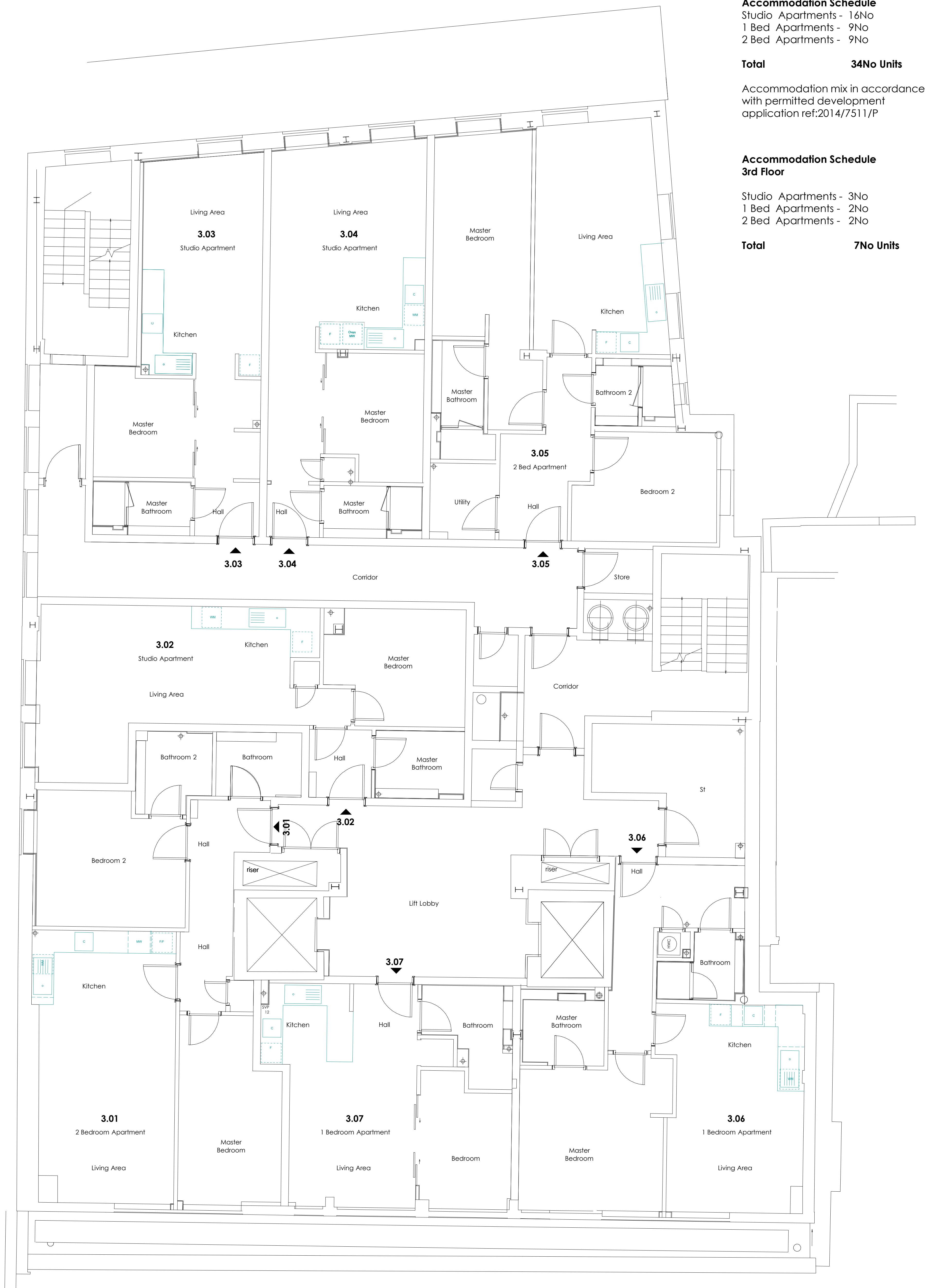
Proposed Third Floor Plan
