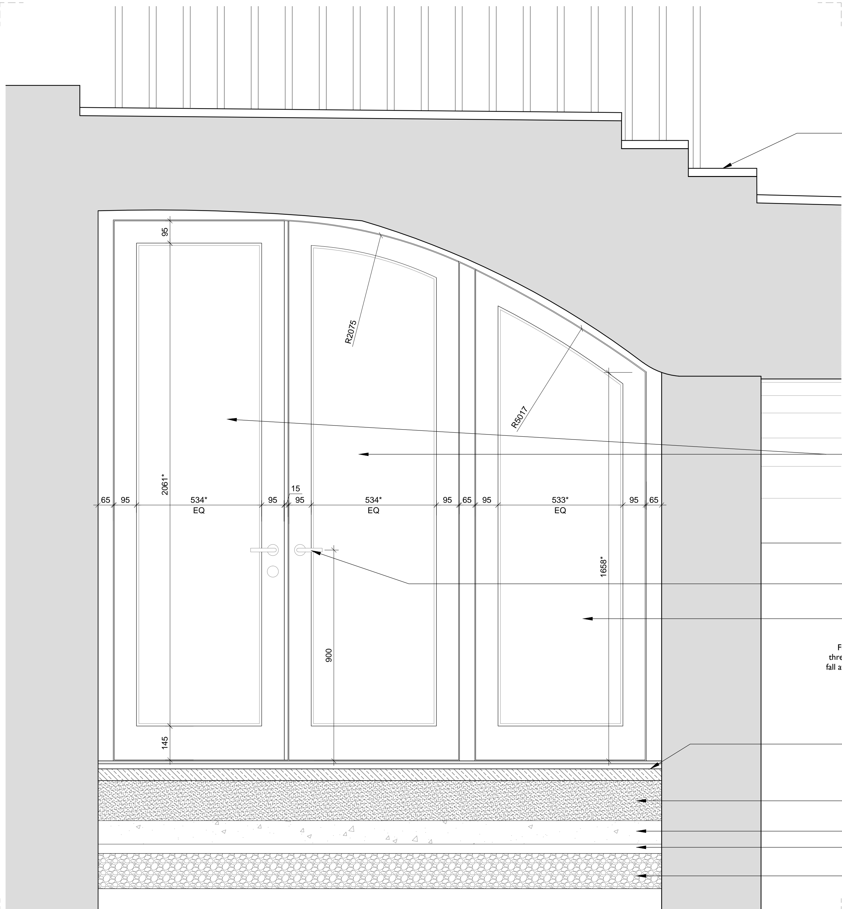
02 External Glazed Screen Elevation
