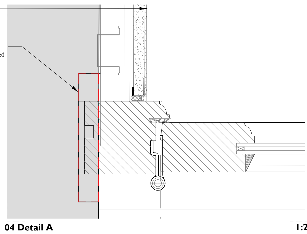
04 Detail A
