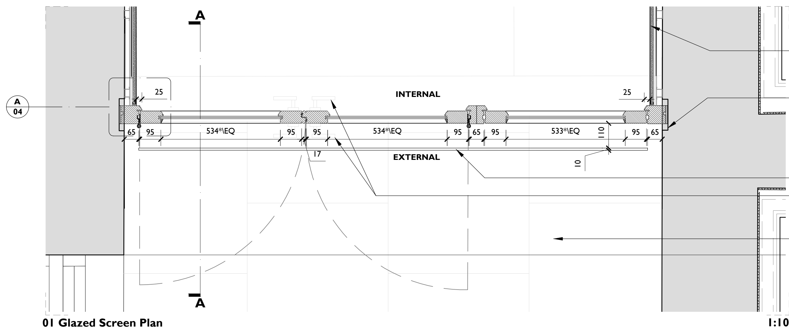
01 Glazed Screen Plan
