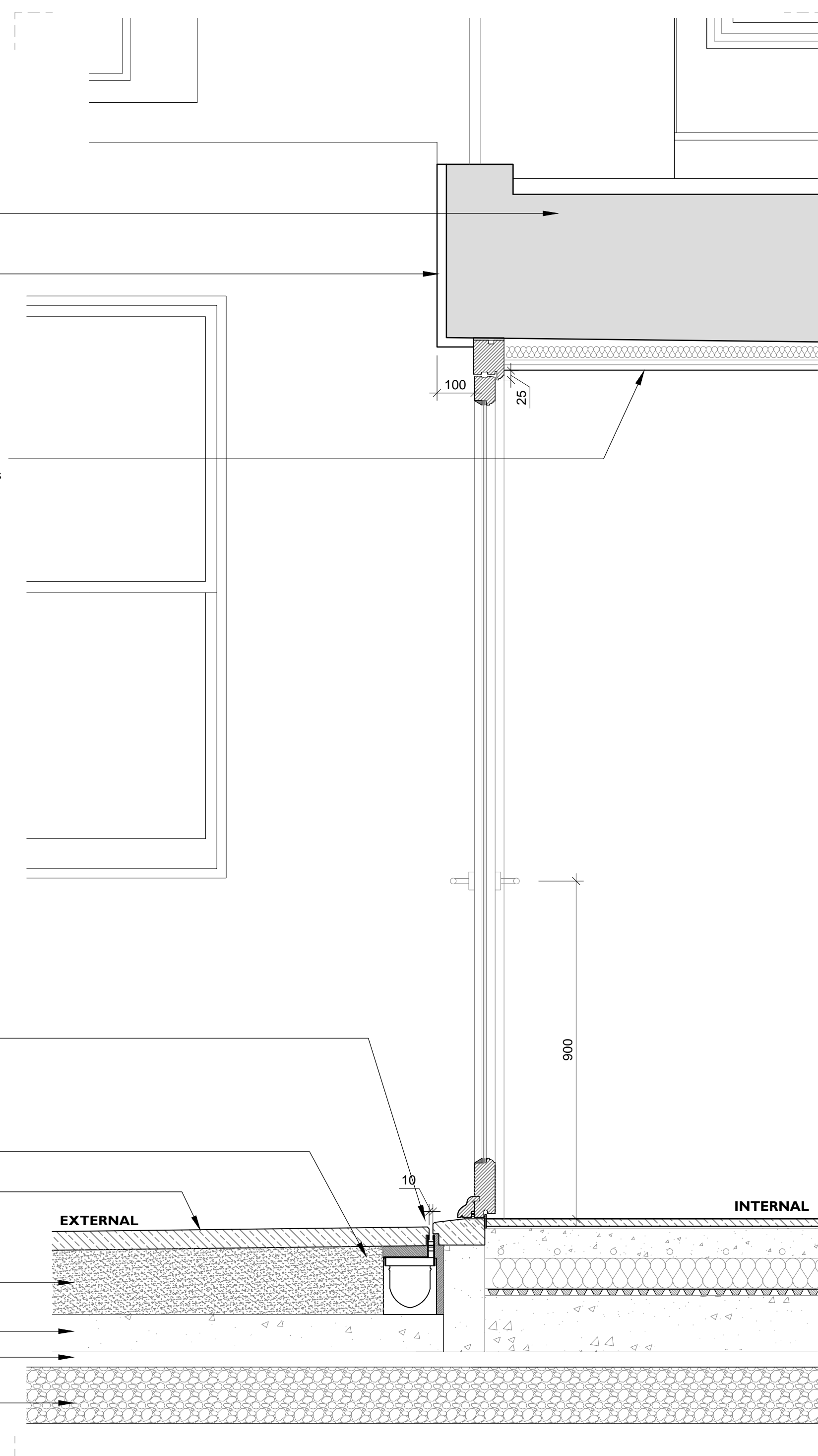
03 Section AA
