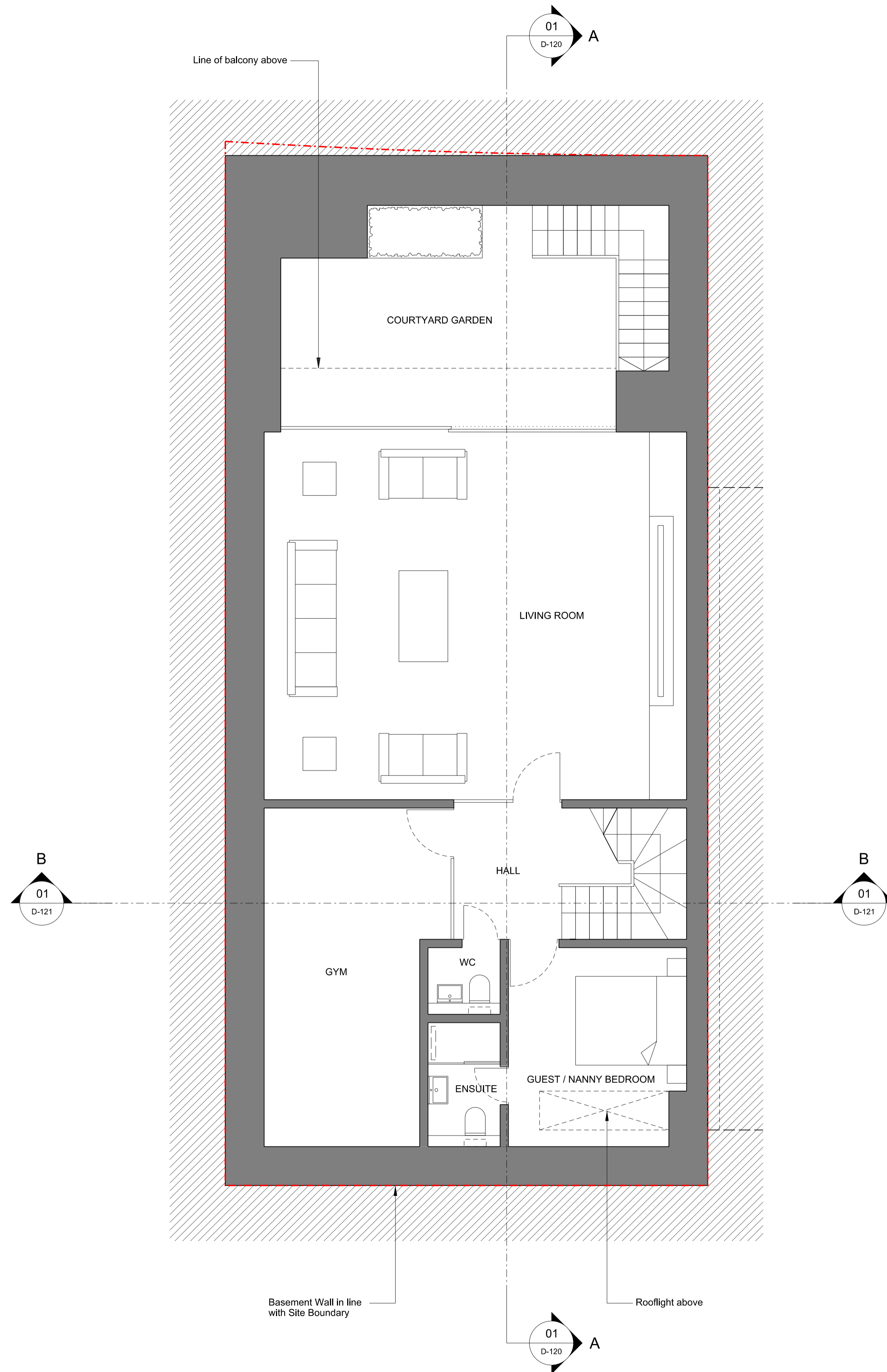
02 BASEMENT PLAN D-110 PROPOSED
