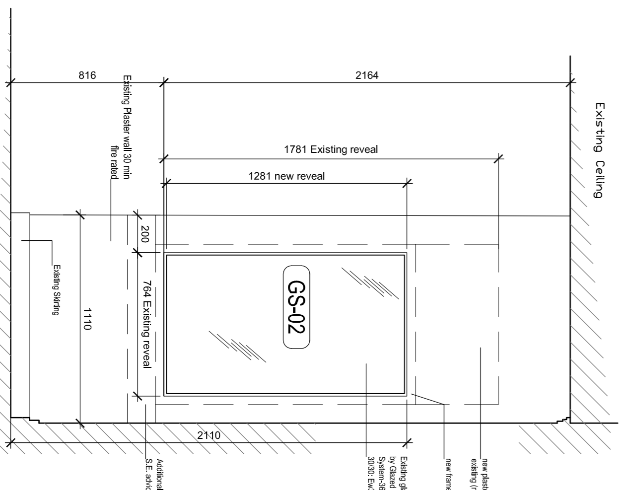
2. Library partition wall detail elevation A Scale 1:20
