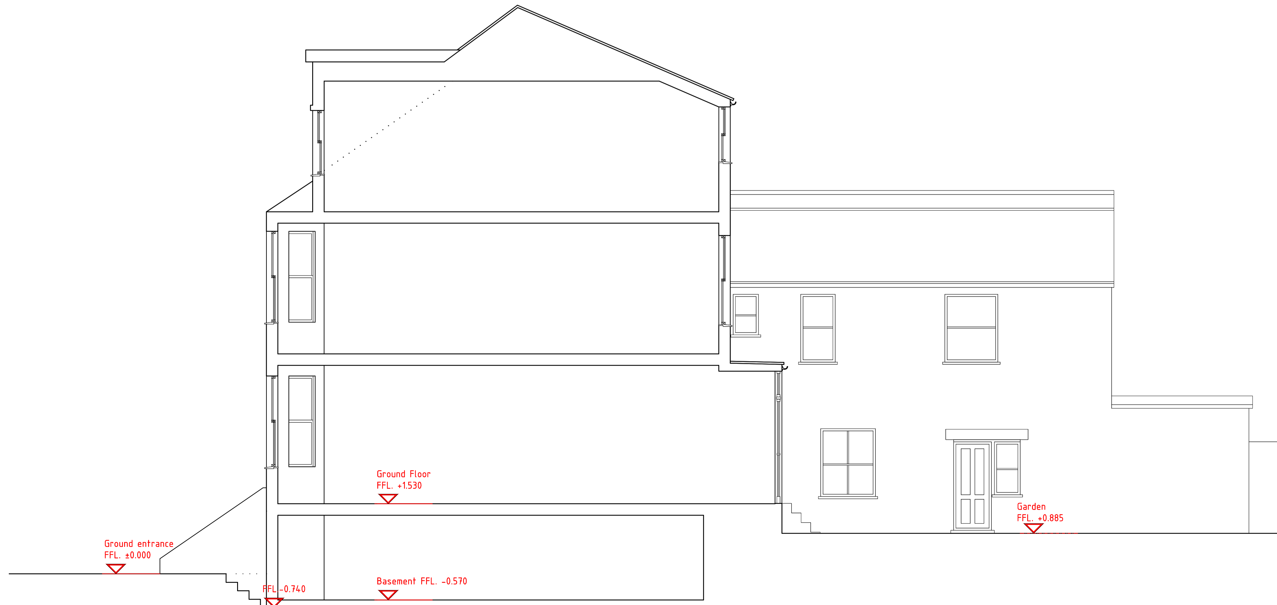
SECTION WITH WINDOWS AS PROPOSED
