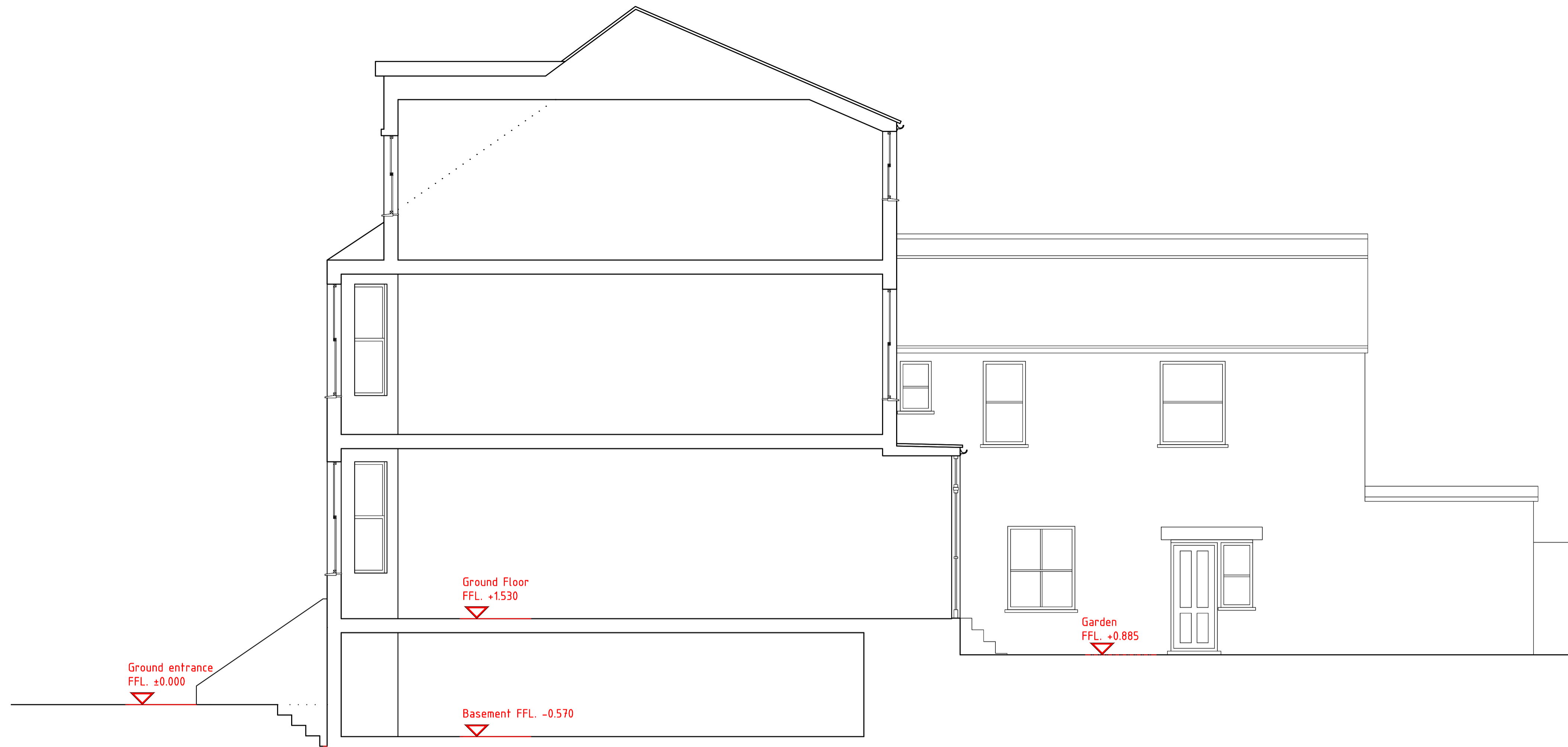
SECTION WITH WINDOWS AS EXISTING
