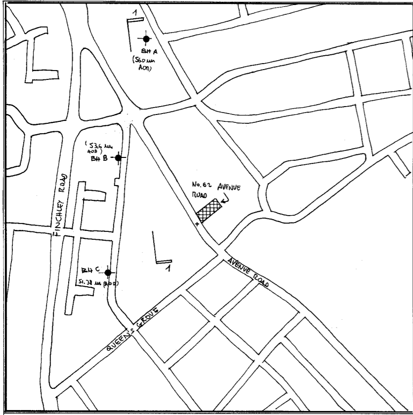
BOREHOLES LOCATION PLAN (1:2000)
