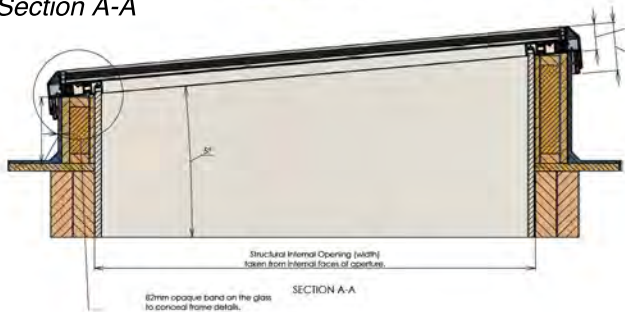
Detail sections of skylight
