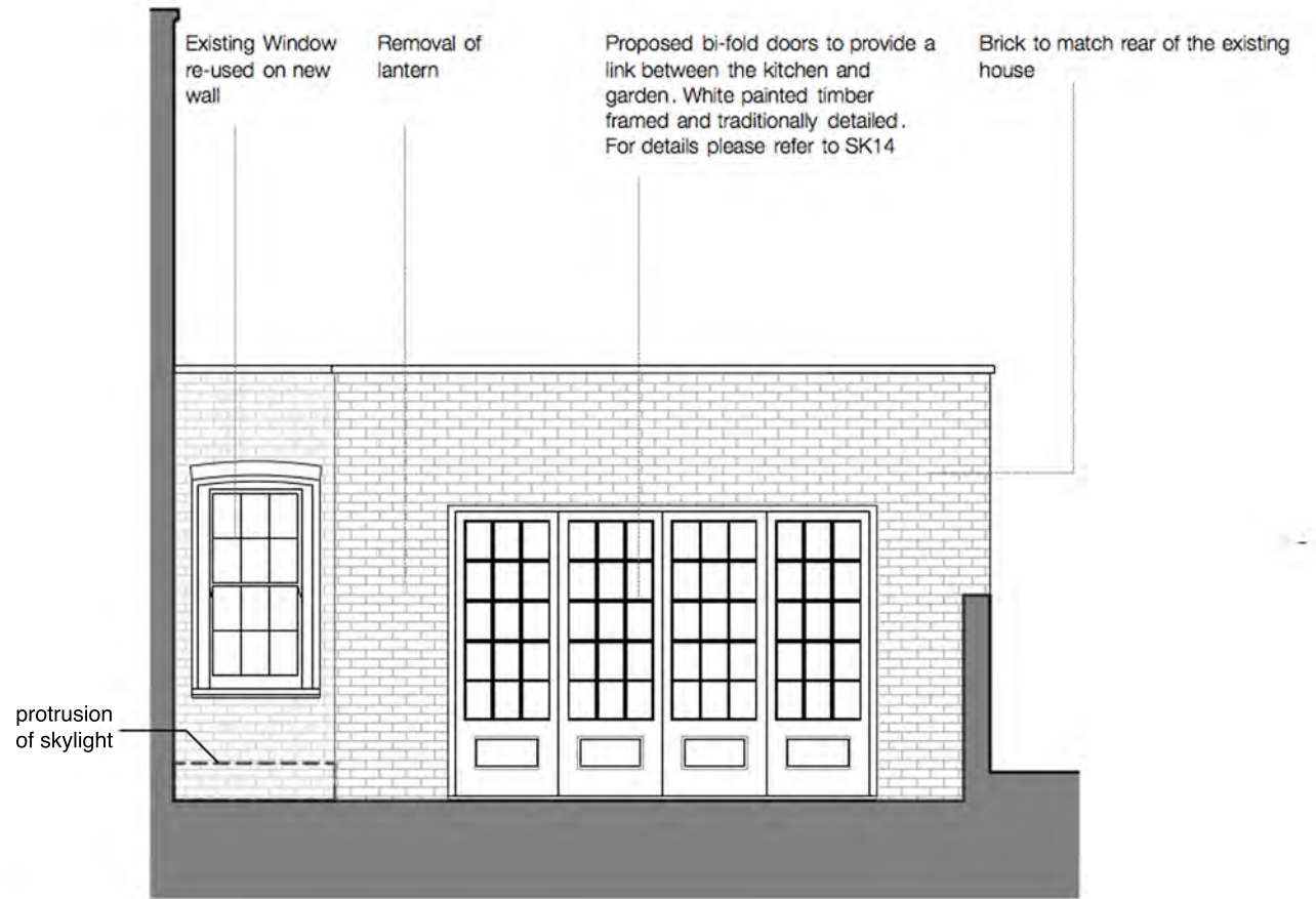
North- West Elevation D
