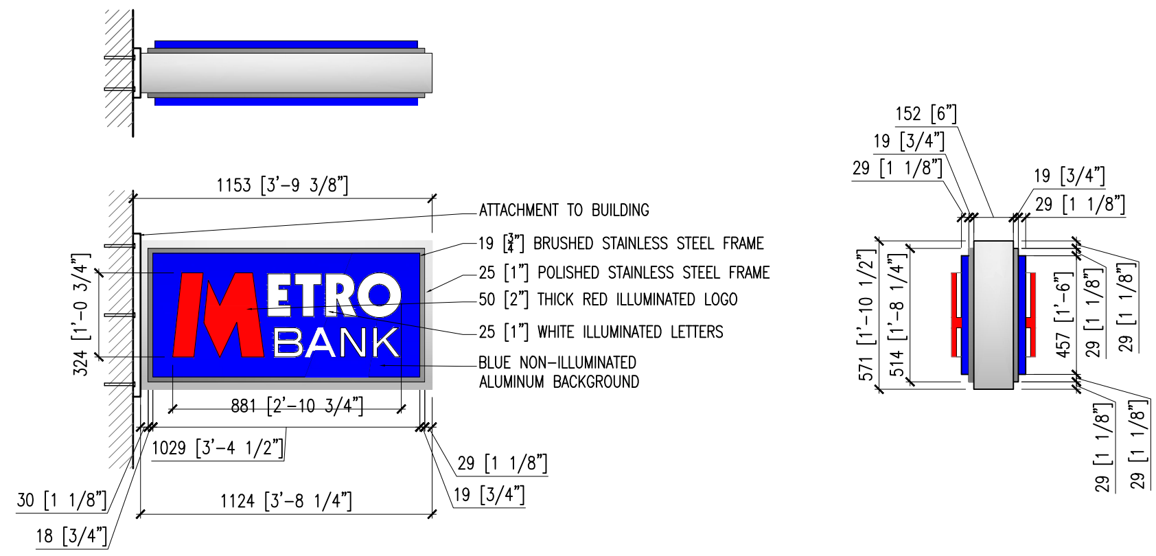
① PROPOSED BLADE SIGNAGE DETAILS
