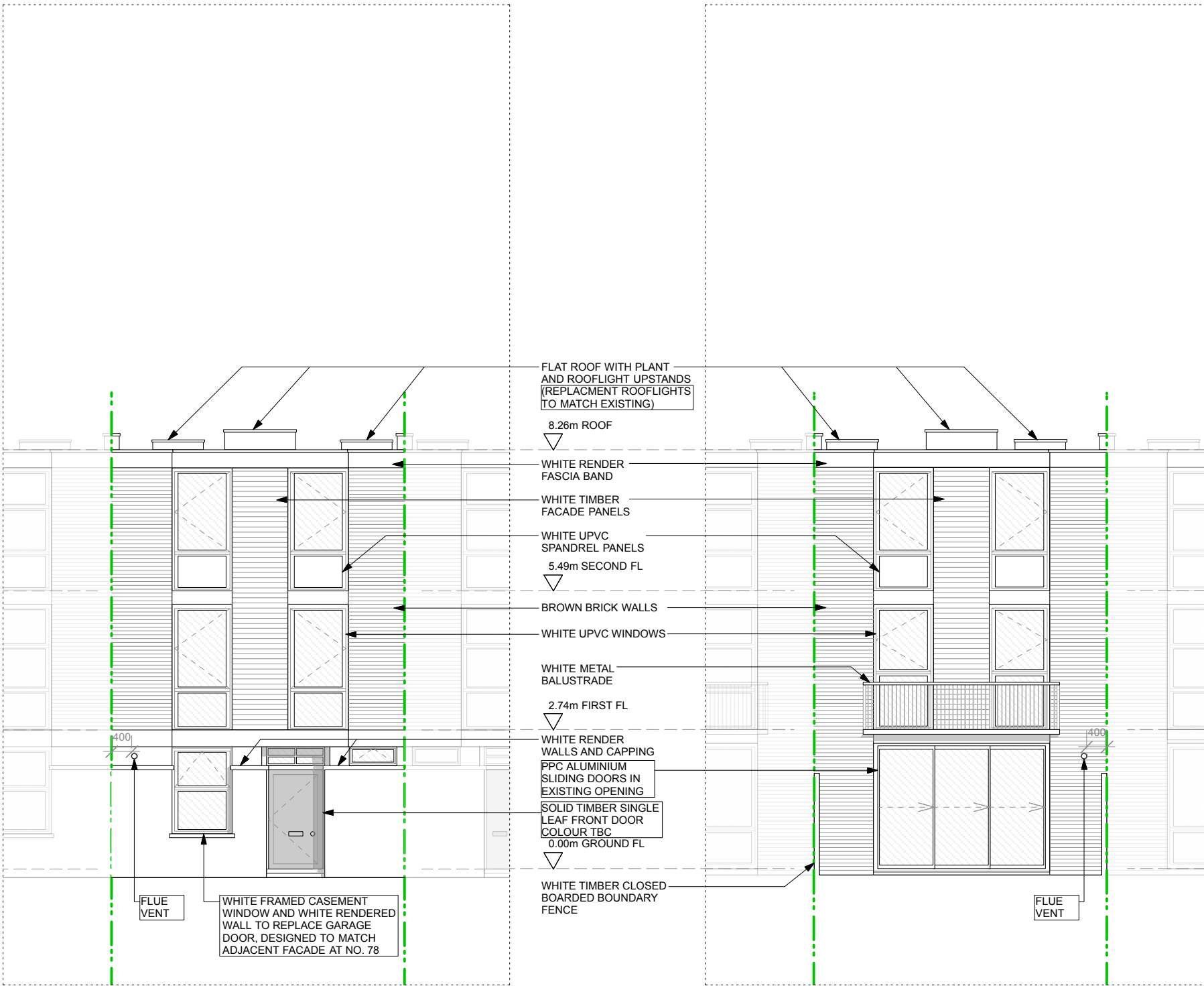
PROPOSED FRONT ELEVATION @ SCALE 1:100
