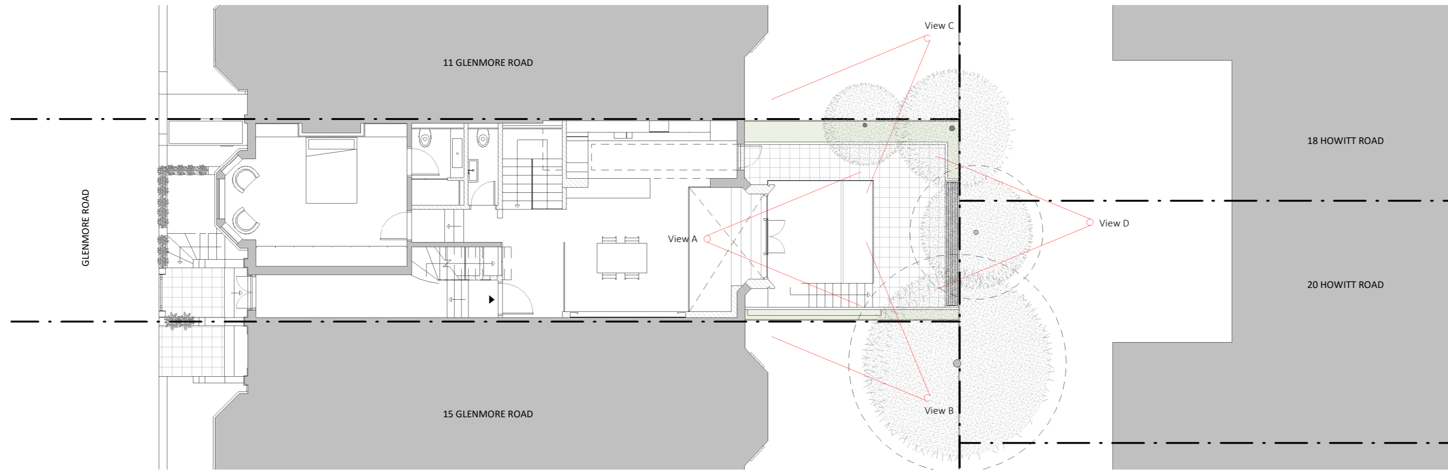
1 Proposed Neighbourhood Plan 1 : 100
