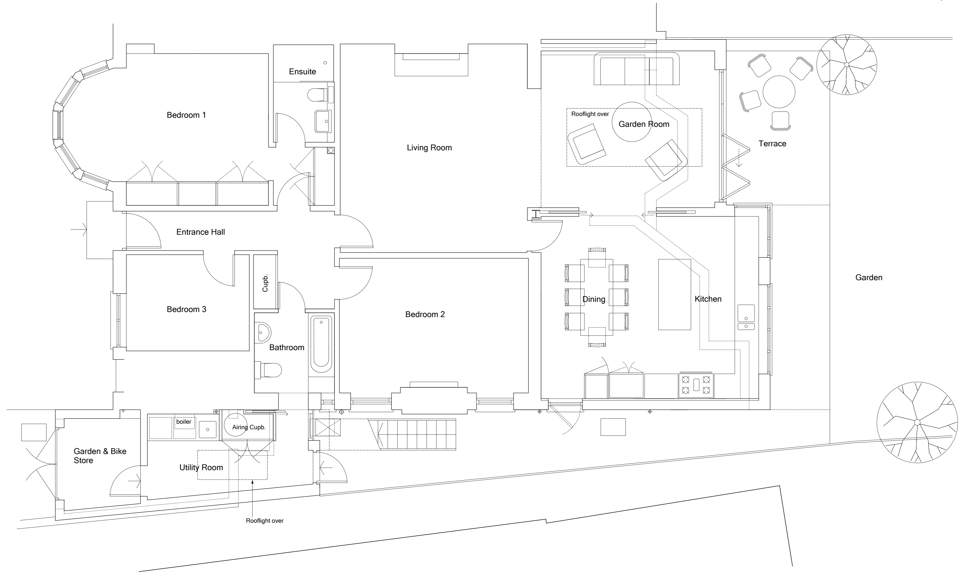
Proposed Ground Floor Plan scale 1:50 @ A2
