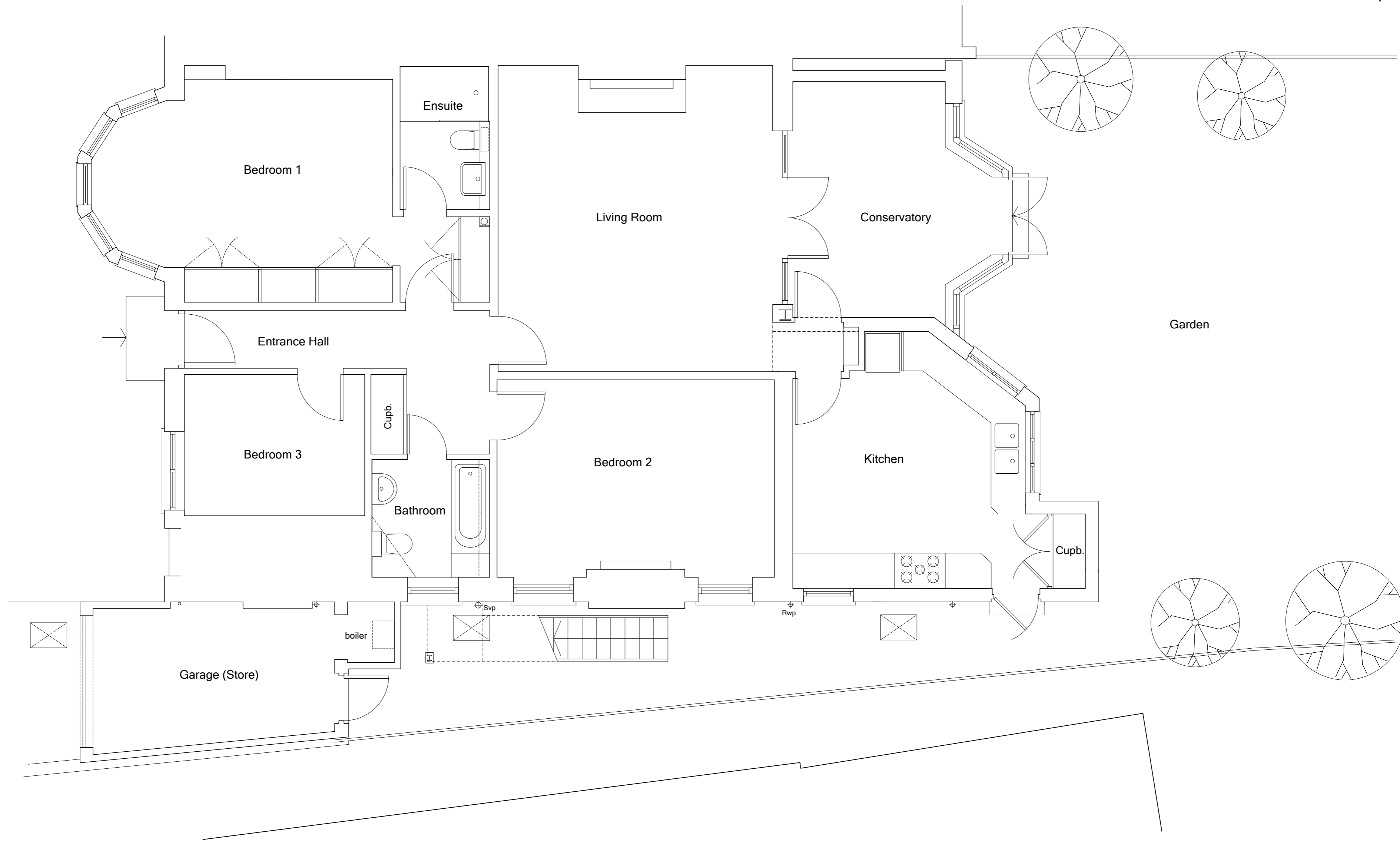
Existing Ground Floor Plan scale 1:50 @ A2
