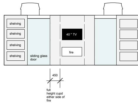
ELEVATION CC
