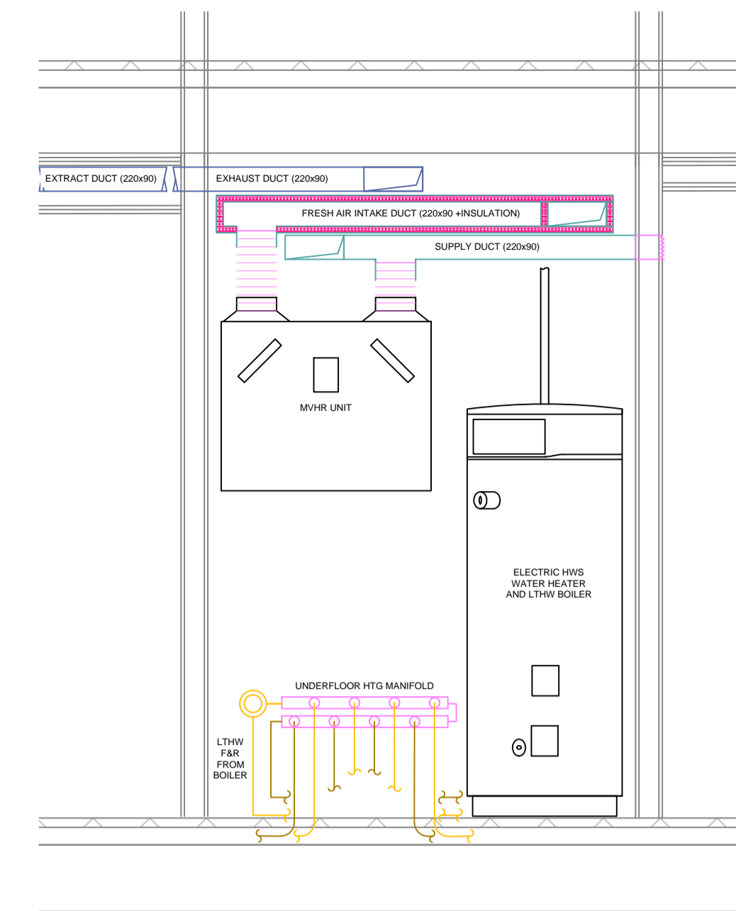
D SERVICE CUPBOARD DETAIL Scale: 1:20
