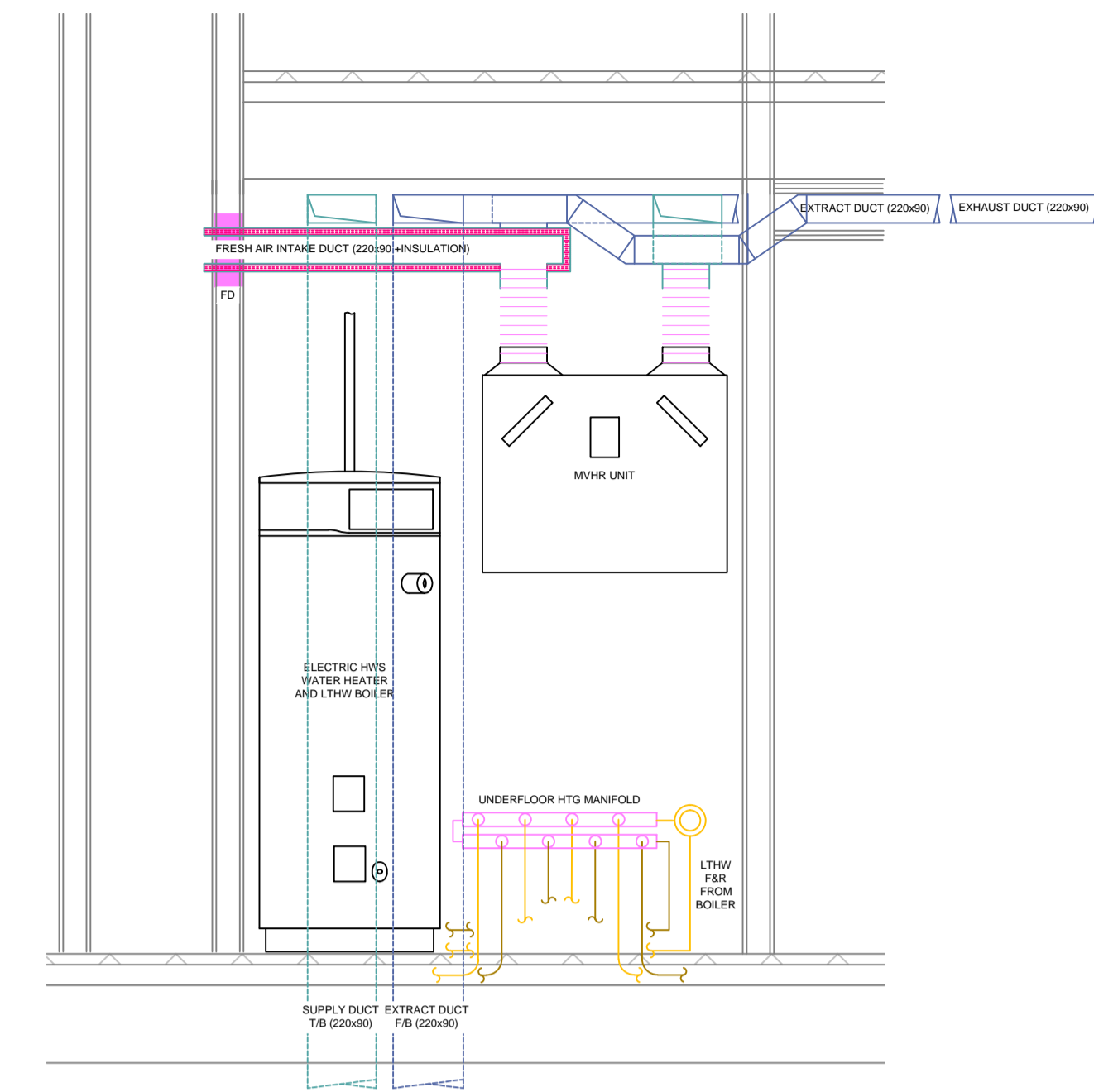
D SERVICE CUPBOARD DETAIL Scale: 1:20
