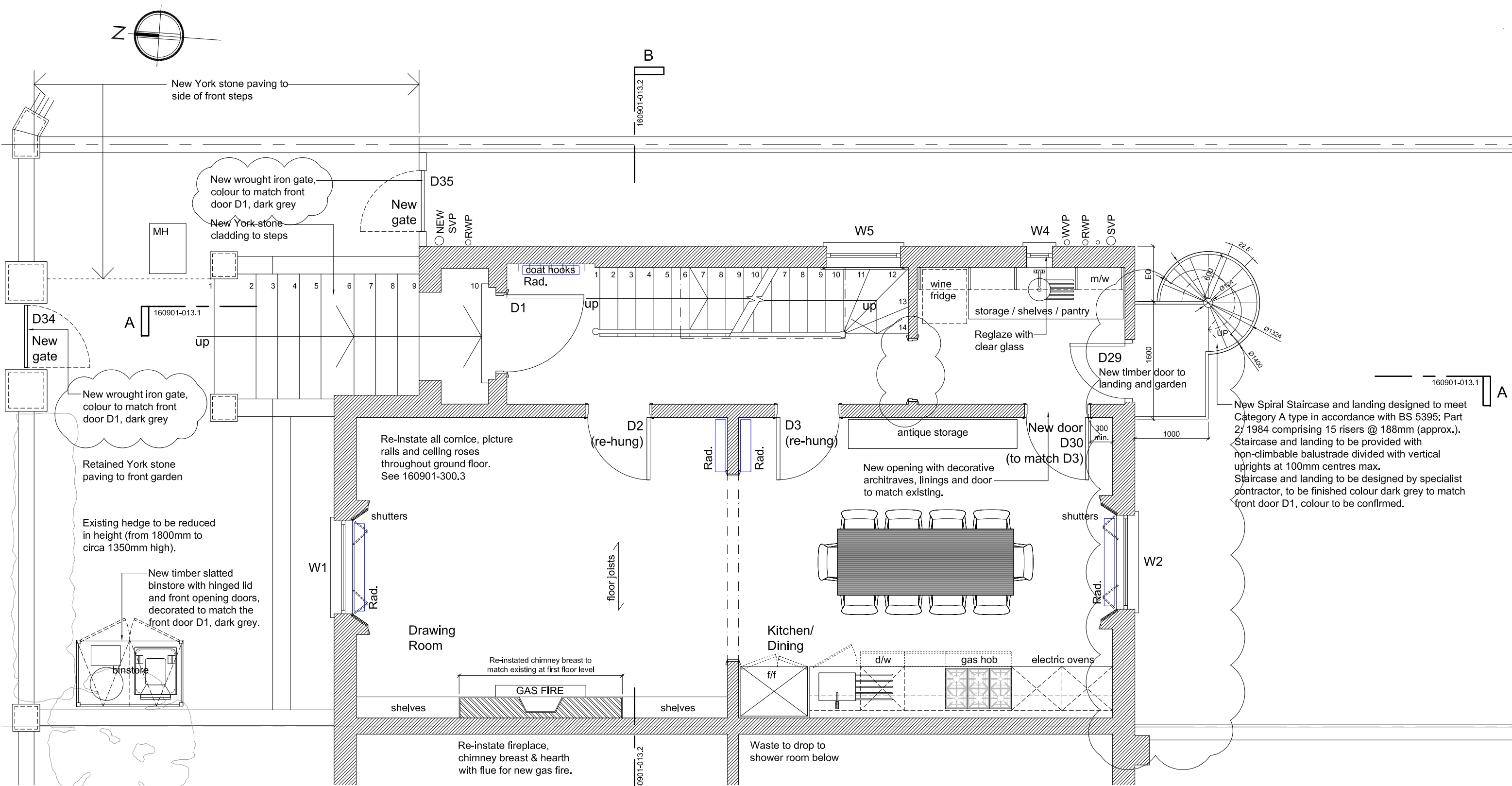
Ground Floor Plan as Proposed Scale 1:50 @ A3
