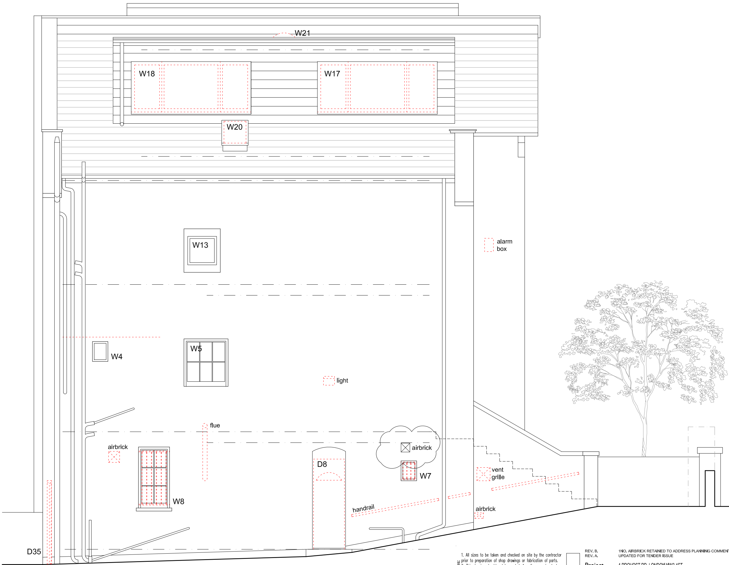
Flank (side) Elevation as Existing - Downtakings
