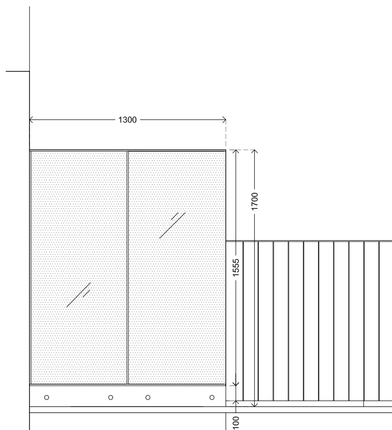
Proposed Terrace Privacy Screen Elevation
