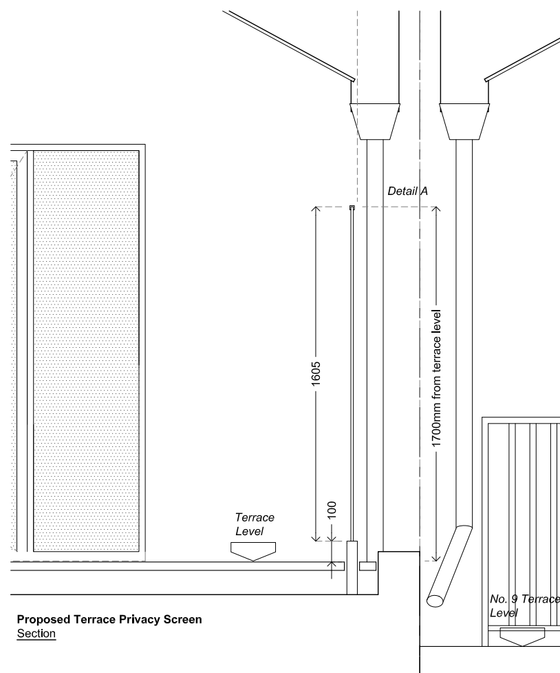
Section Detail A Terrace Privacy Screen
