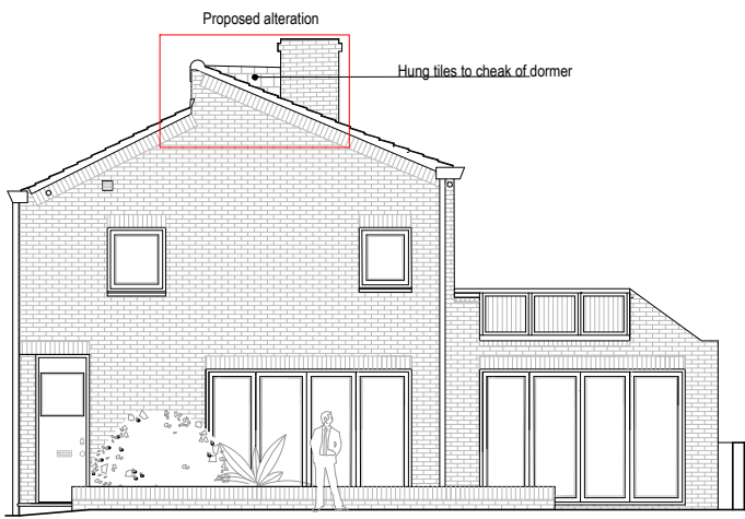
SOUTH-EAST ELEVATION
