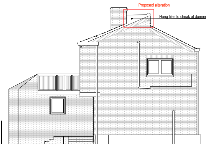
NORTH-WEST ELEVATION
