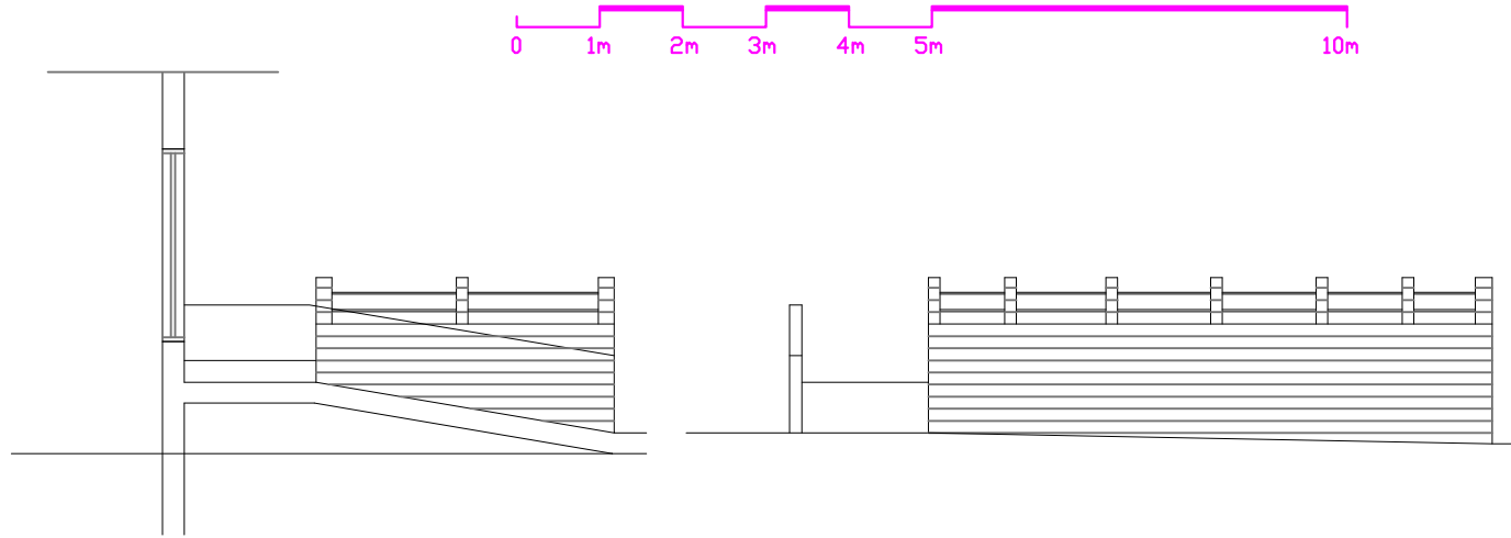
LEFT SIDE ELEVATION Scale-1:100@A3
