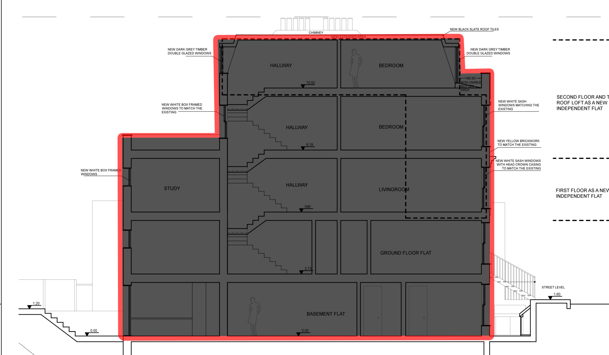
2016 Volume of 90 Torriano Avenue Proposal
