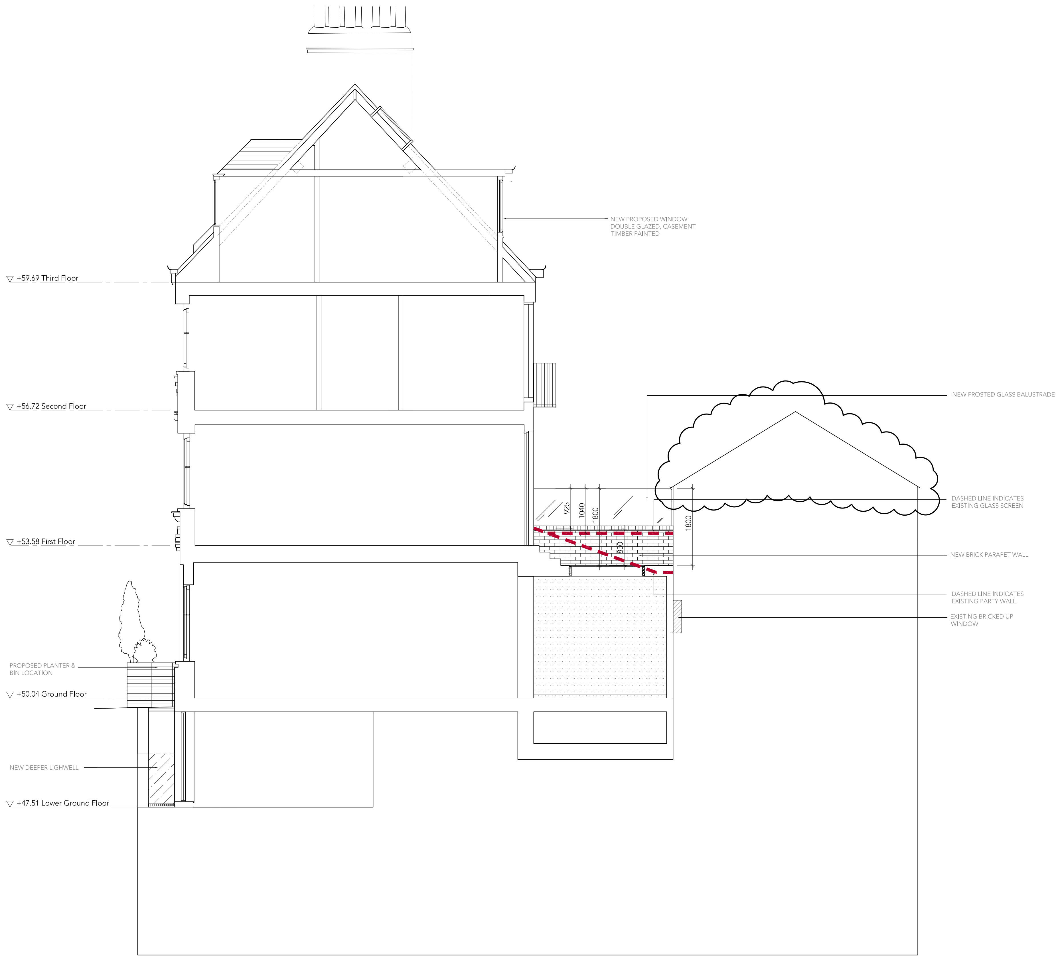
1 Section A scale 1:50
