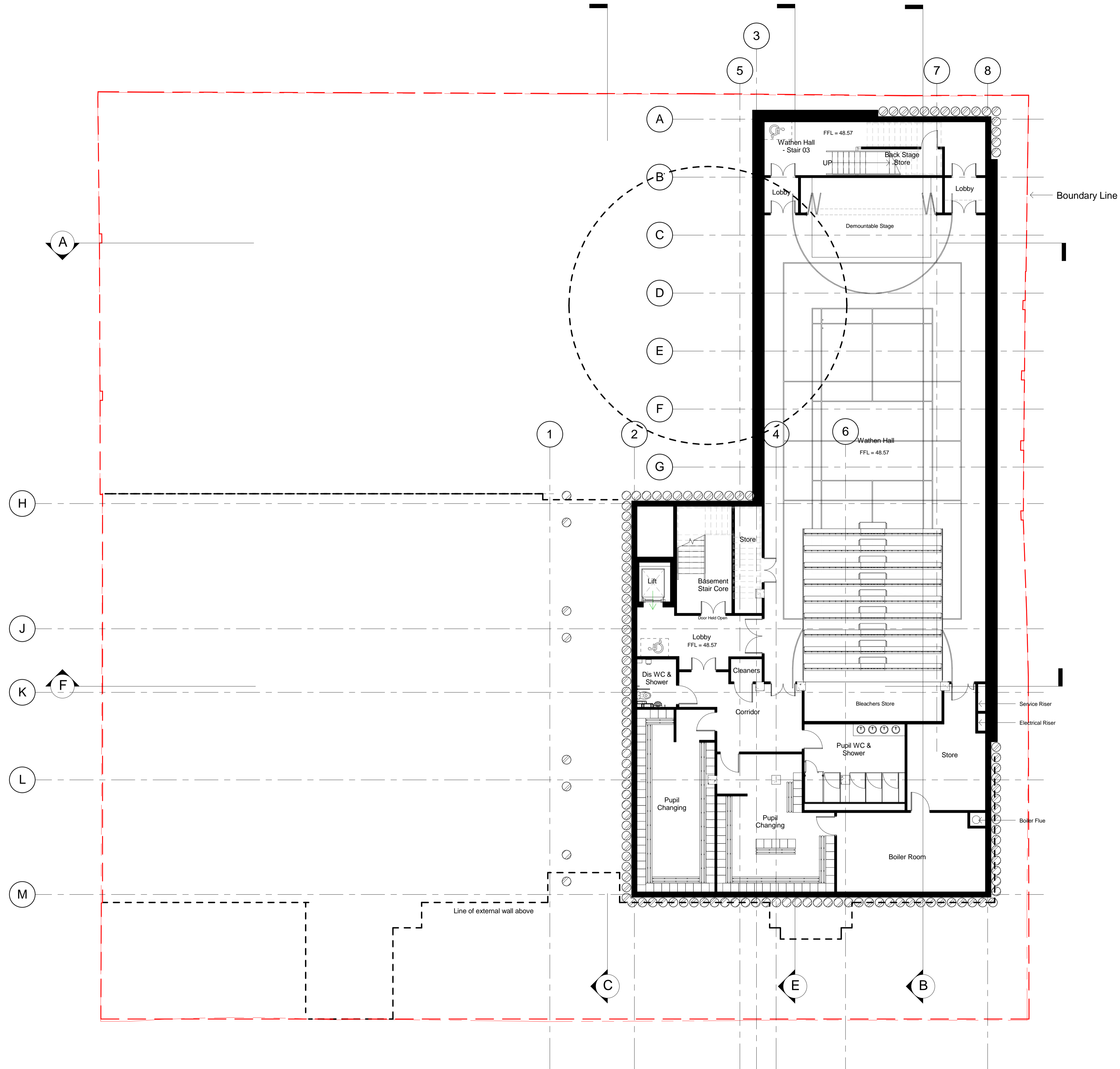
Proposed Planning L-04 Basement 02 1 : 100
