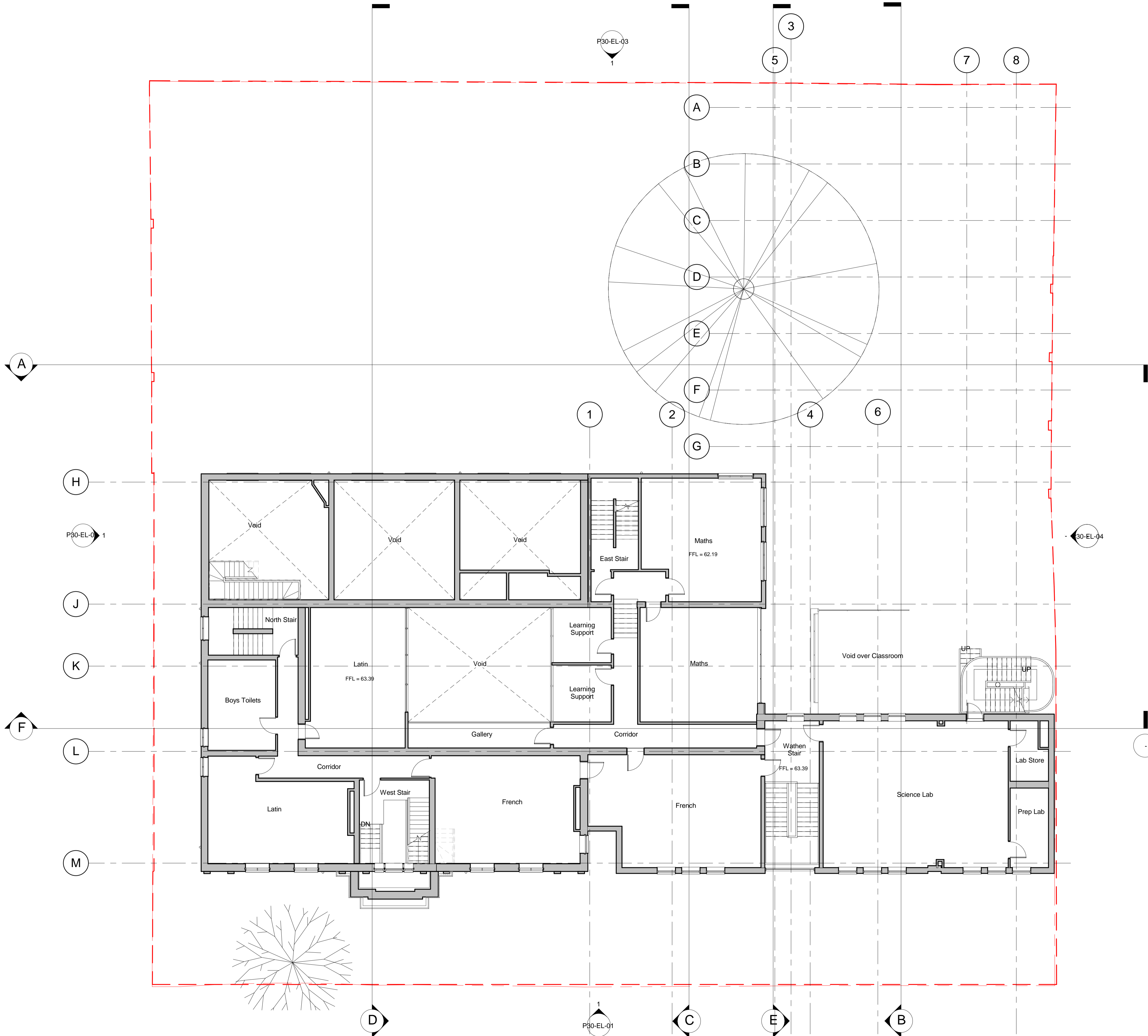
Existing L01 First Floor 1 : 100
