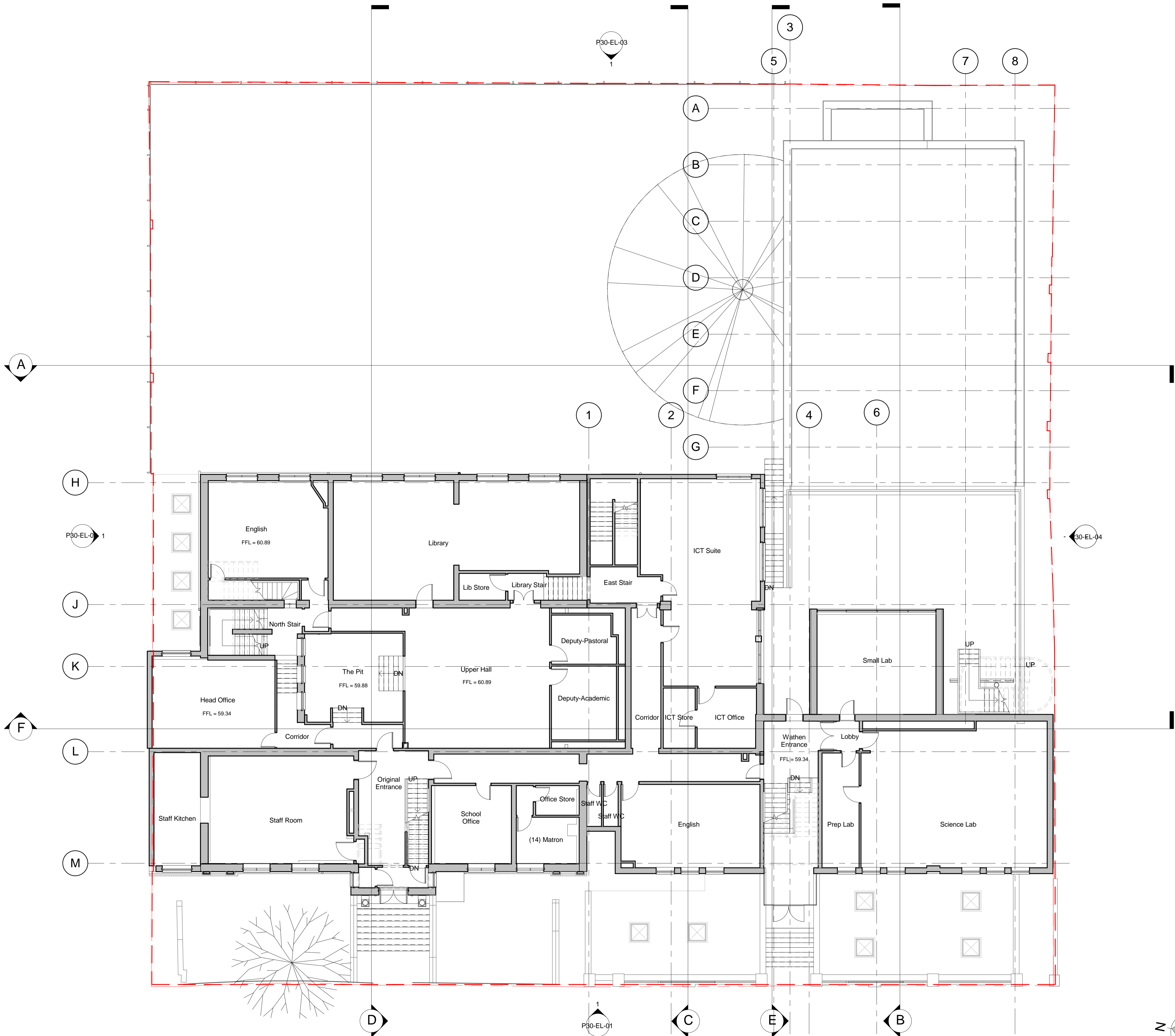
Existing L00 Ground Floor 1 : 100
