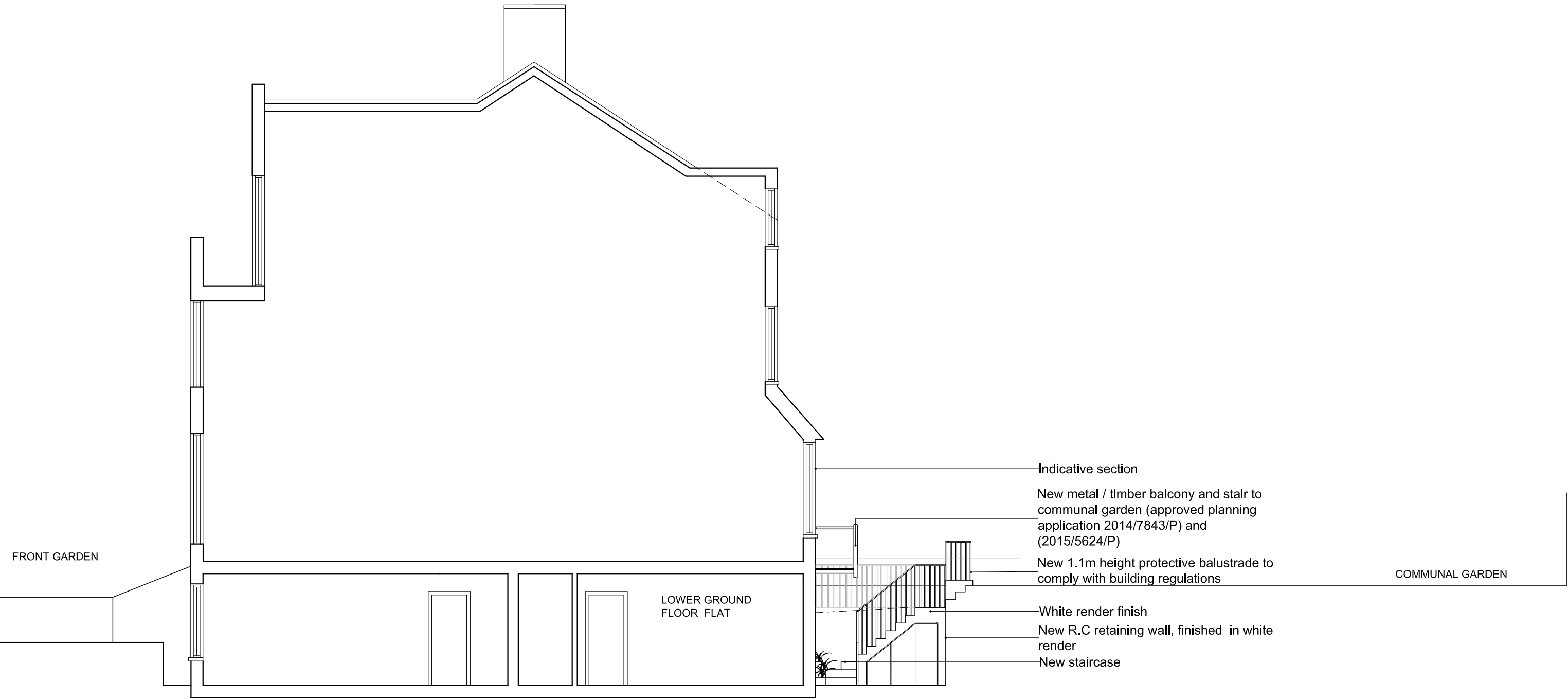
SECTION BB
