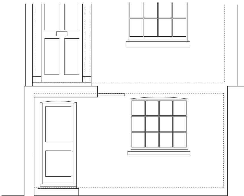
EXISTING FRONT AREA ARRANGEMENT (RAILINGS/BALUSTRADING OMITTED FOR CLARITY)
