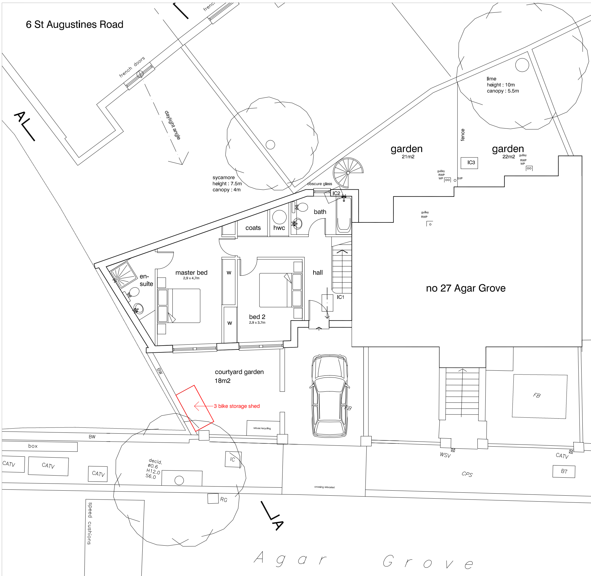
site plan as proposed
