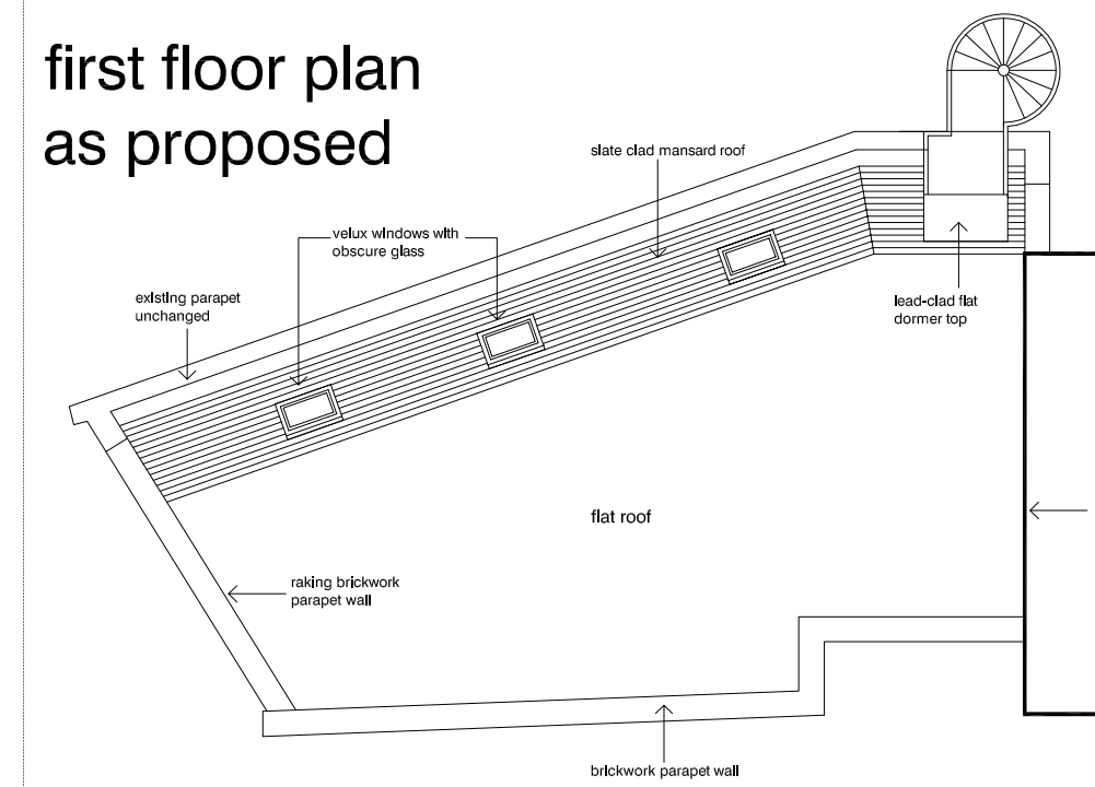
roof plan as proposed
