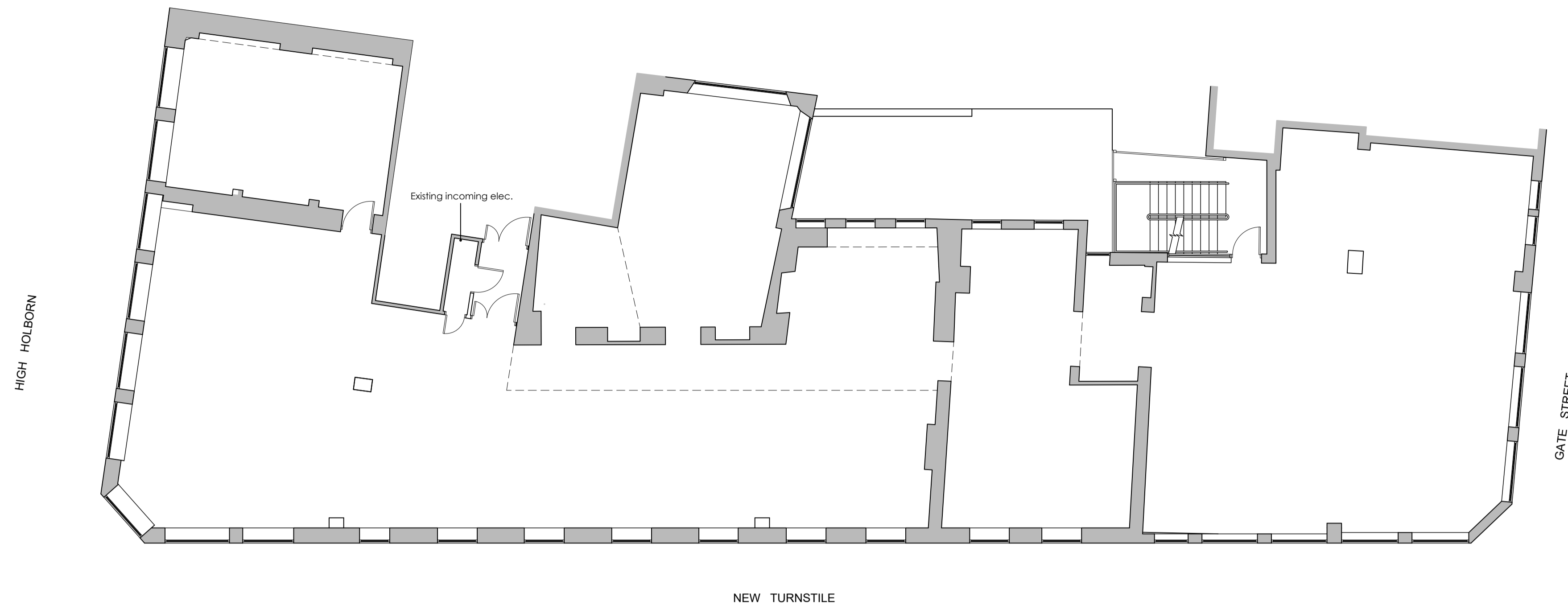
FIRST FLOOR PLAN AS EXISTING
