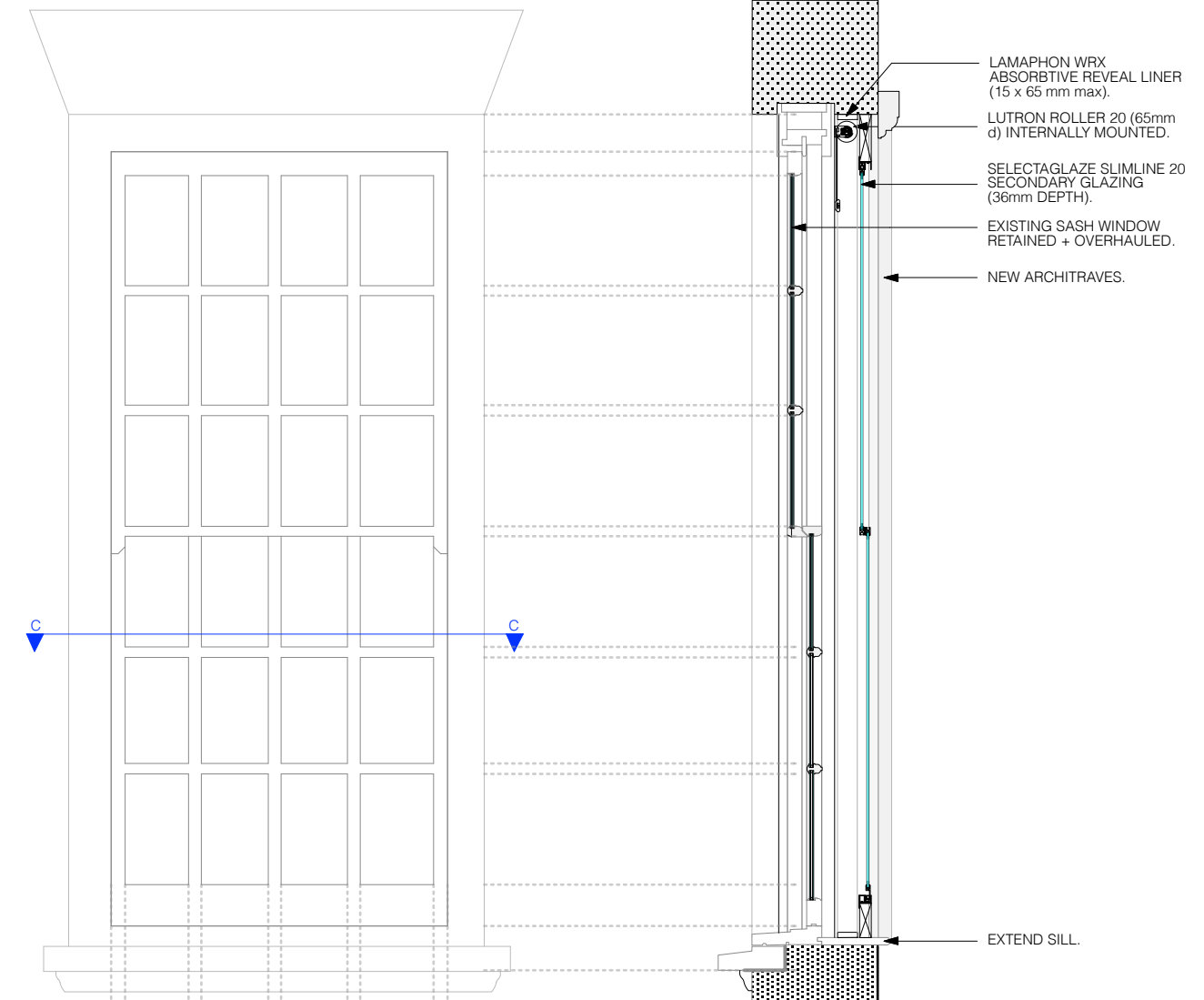
EXTERNAL ELEVATION OF PROPOSED WINDOW TYPE 2.
