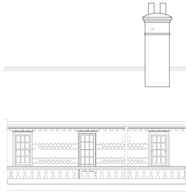
EXISTING MAIN TERRACE ELEVATION 01 1:100 @ A3
