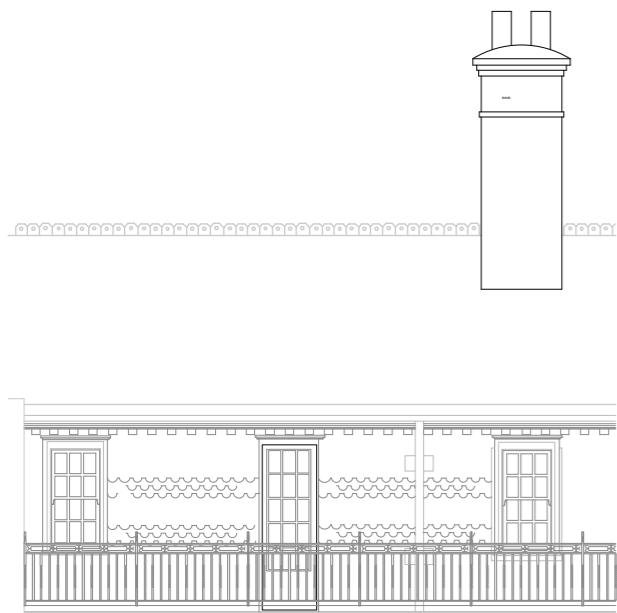
PROPOSED MAIN TERRACE ELEVATION 01 1:100 @ A3
