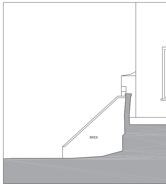
2 Section AA showing buttress 1:50 @ A1
