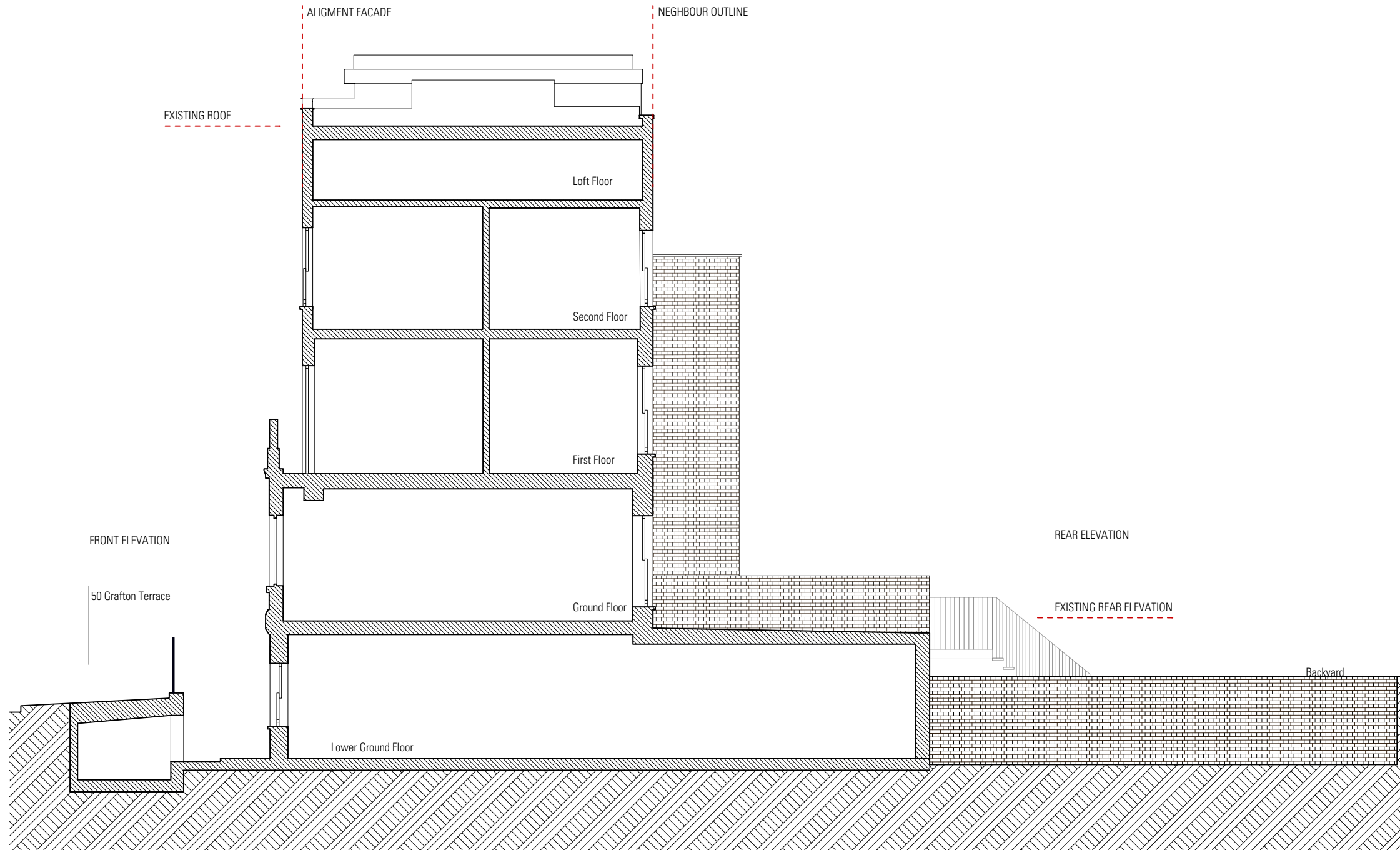
2 48 Grafton Terrace Section Scale 1:100@A3
