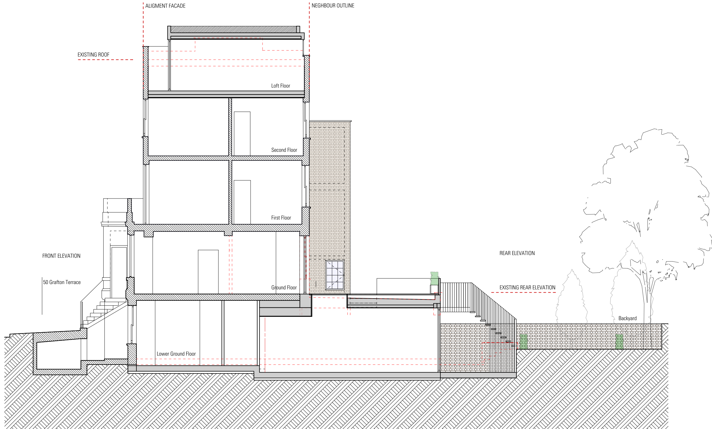
2 Long Section Scale 1:100@A3
