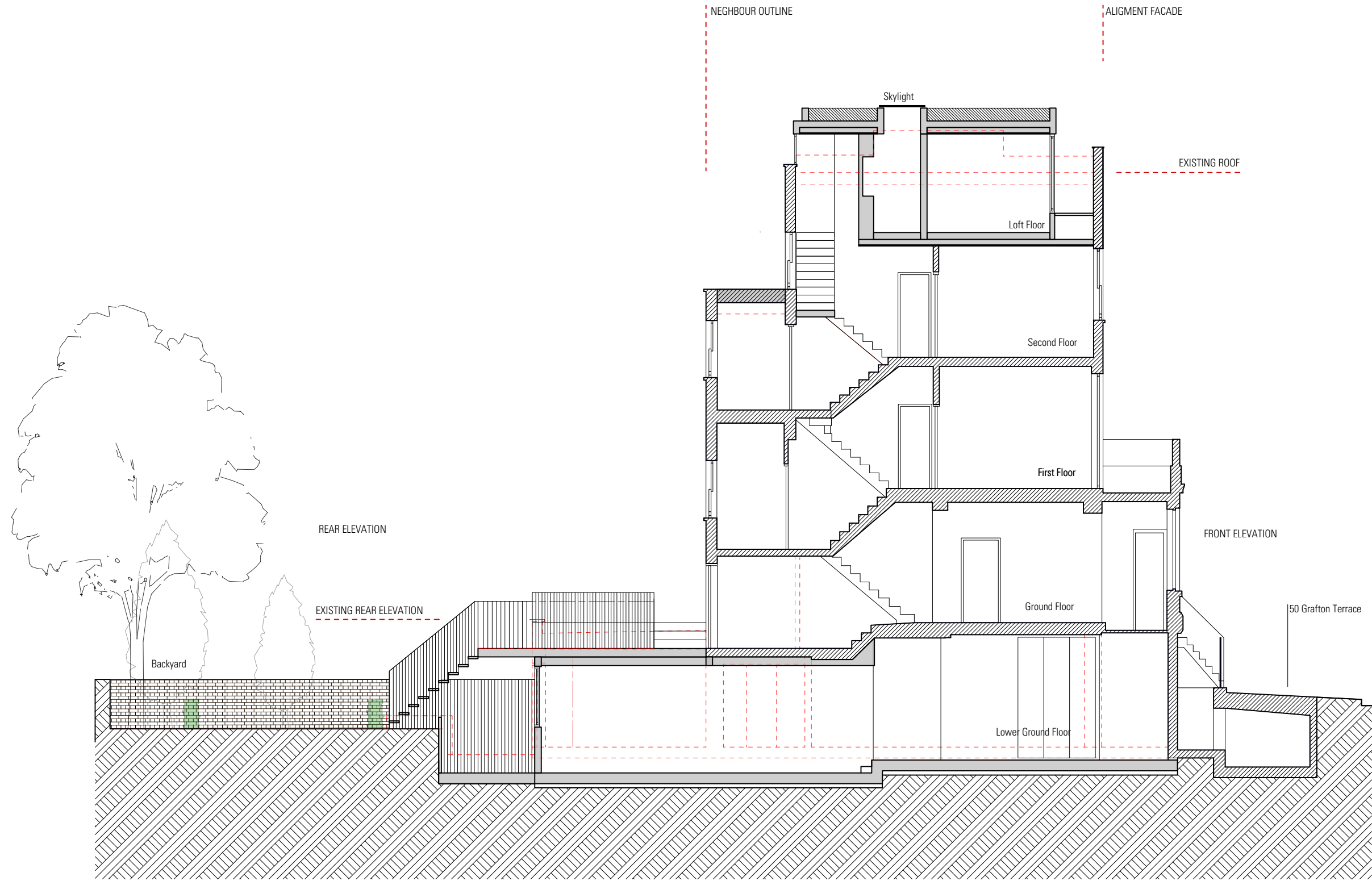
1 Long Section Scale 1:100@A3
