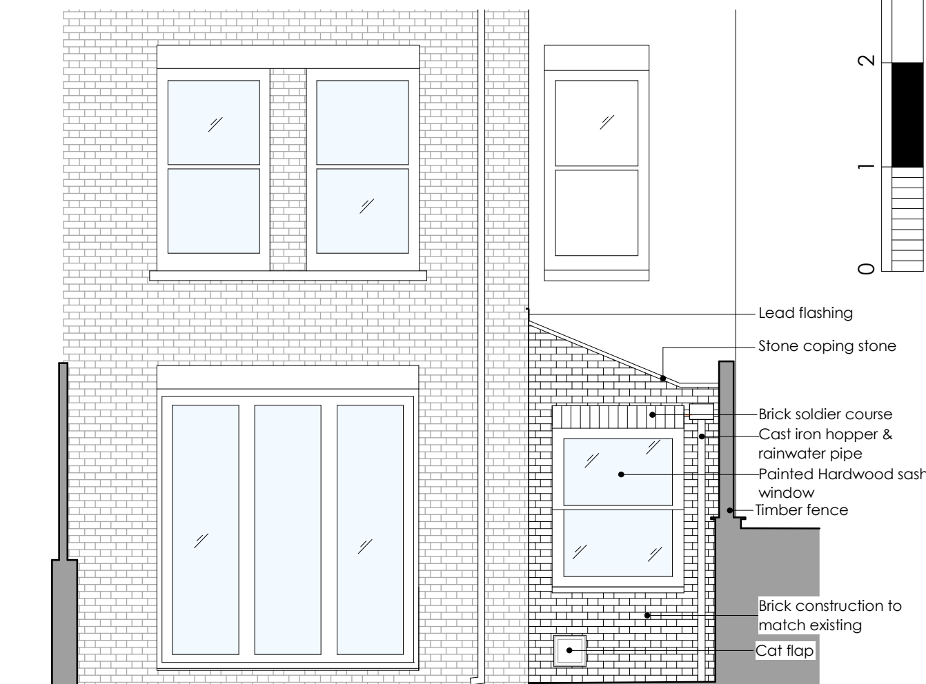
1. PROPOSED REAR ELEVATION
