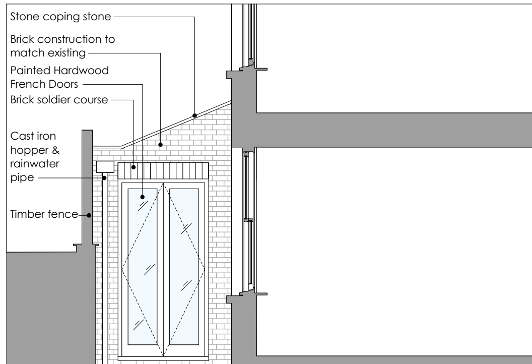
4. PROPOSED SIDE ELEVATION
