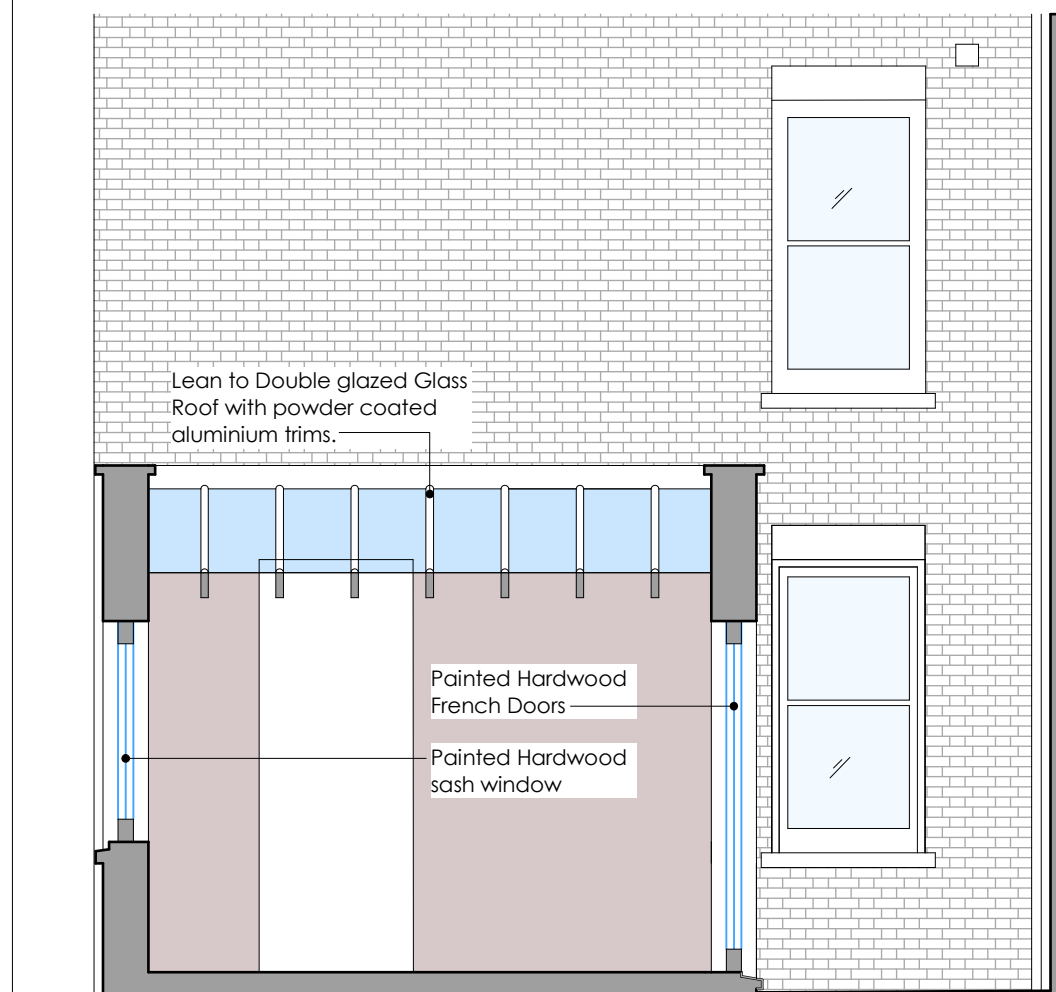
3. PROPOSED SIDE ELEVATION
