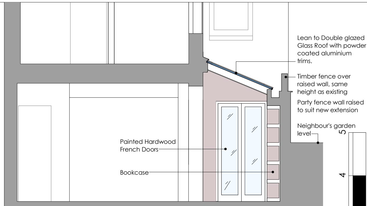
2. PROPOSED SECTION 2-2
