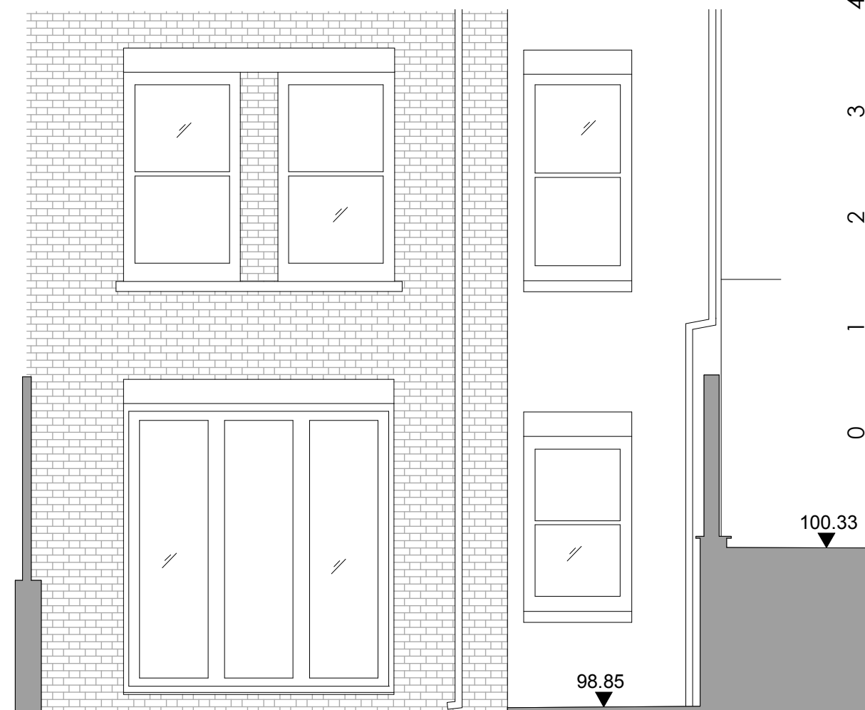
2. EXISTING SECTION 2-2
