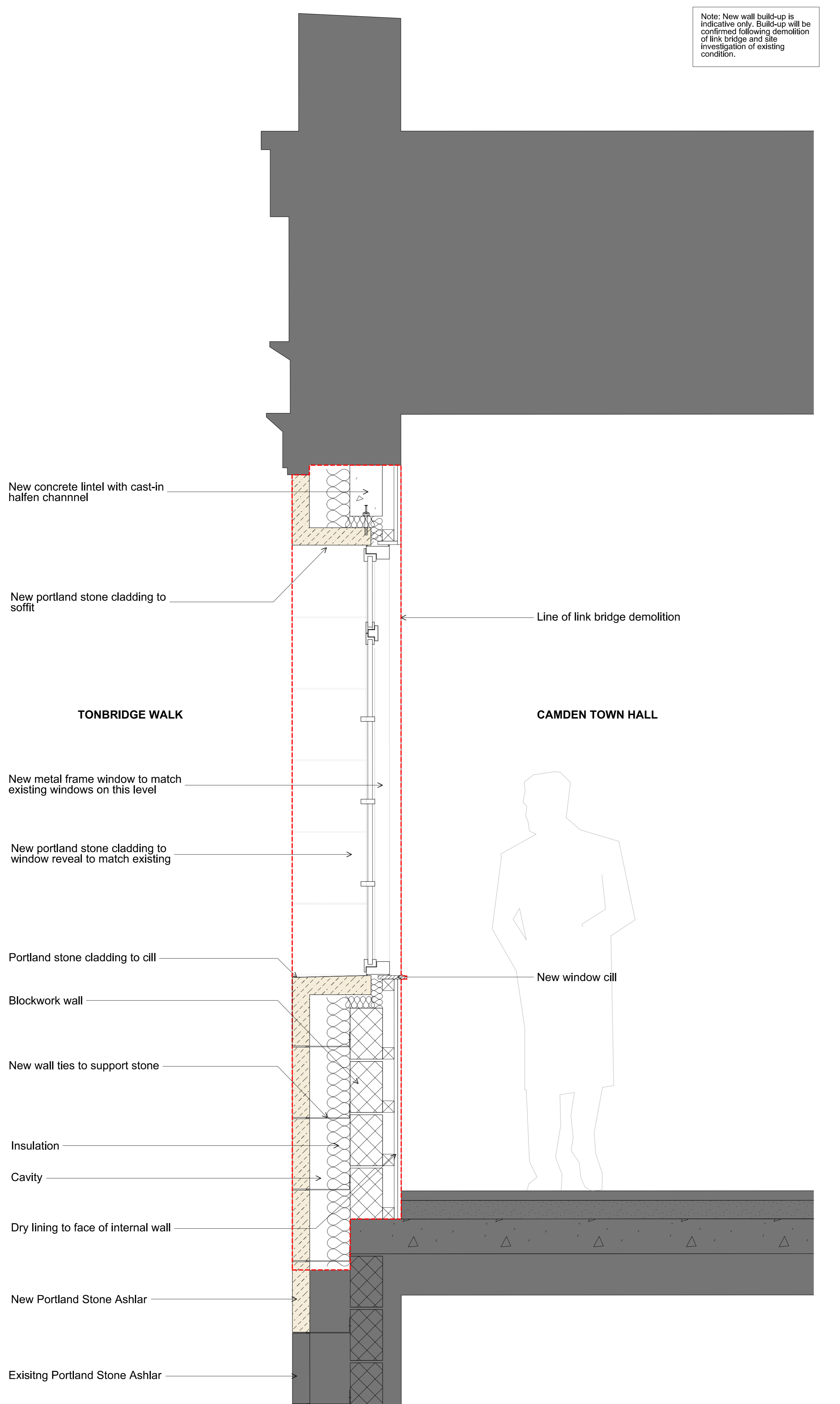
A Section 1:10
