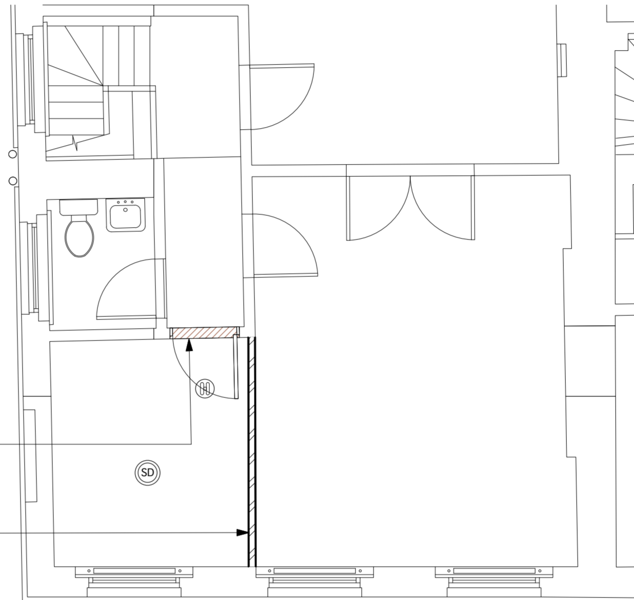
THIRD FLOOR SCALE 1:50
