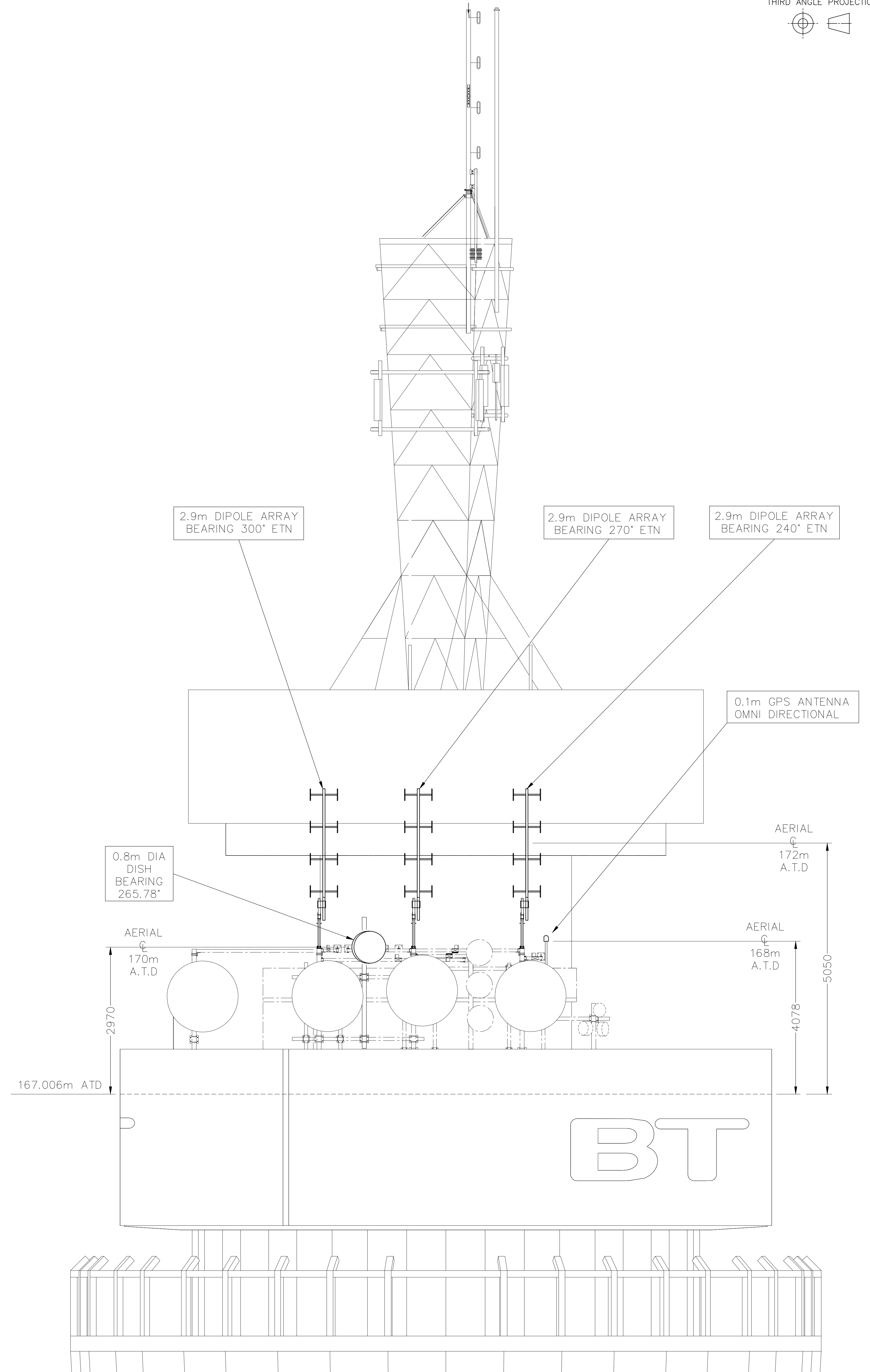
ENLARGED PART ELEVATION VIEW OF TOWER FACING WEST AT 167.006m ATD SHOWING PROPOSED AERIAL SCALE 1:50
