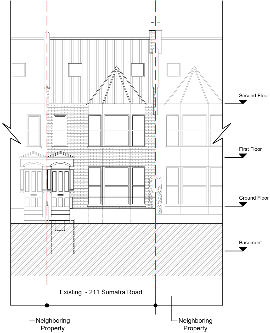
Front Elevation
