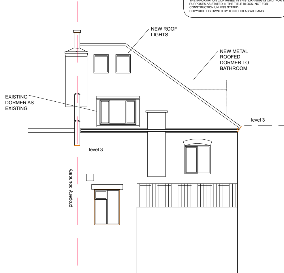
REAR ELEVATION Scale 1:100@A3
